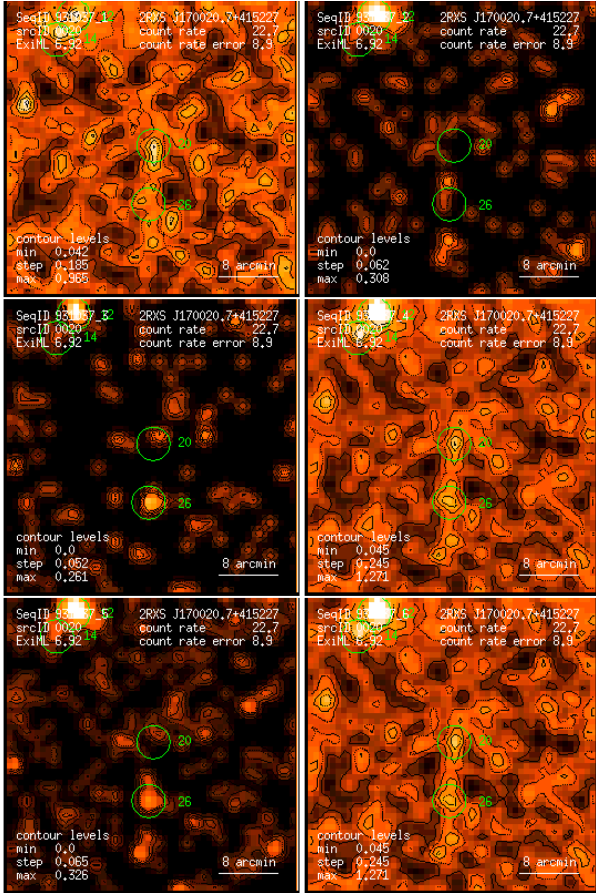
Figure 20: RASS 931037: detection 0020: band rate images, Gaussian filter: (1) PSPC channels 11 – 41, (2) 52 – 90, (3) 91 – 201, (4) 11 – 235, (5) 52 – 201, (6) 11 – 201. Broad band rates in counts/ks. Band rate contour levels in counts/ks/arcmin 2 .
