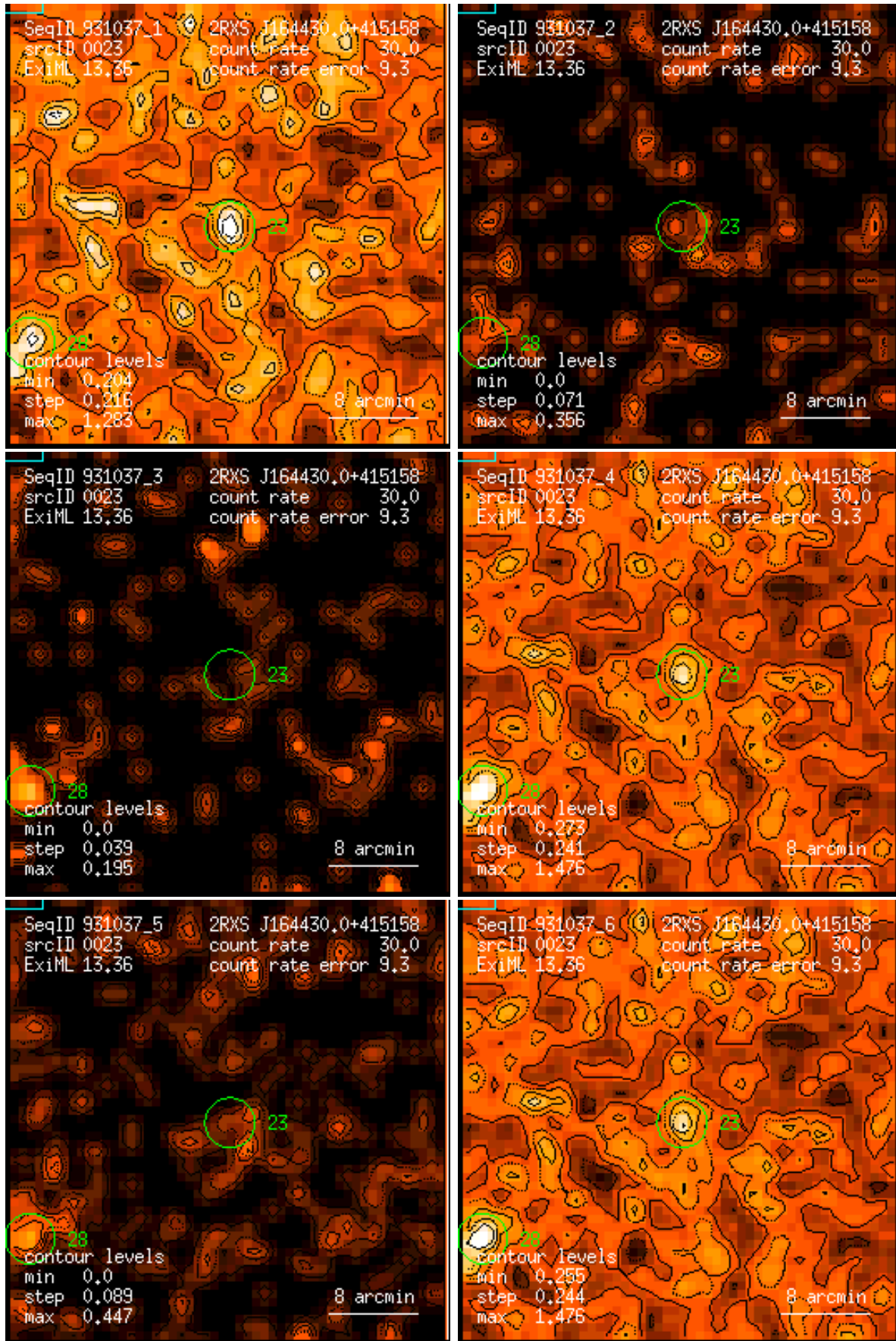
Figure 23: RASS 931037: detection 0023: band rate images, Gaussian filter: (1) PSPC channels 11 – 41, (2) 52 – 90, (3) 91 – 201, (4) 11 – 235, (5) 52 – 201, (6) 11 – 201. Broad band rates in counts/ks. Band rate contour levels in counts/ks/arcmin 2 .
