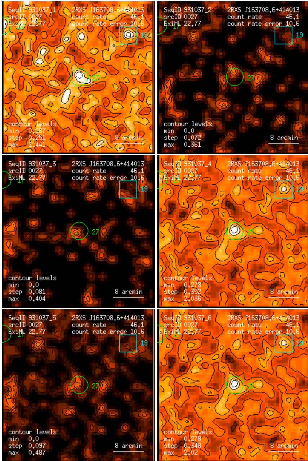
Figure 27: RASS 931037: detection 0027: band rate images, Gaussian filter: (1) PSPC channels 11 – 41, (2) 52 – 90, (3) 91 – 201, (4) 11 – 235, (5) 52 – 201, (6) 11 – 201. Broad band rates in counts/ks. Band rate contour levels in counts/ks/arcmin 2 .
