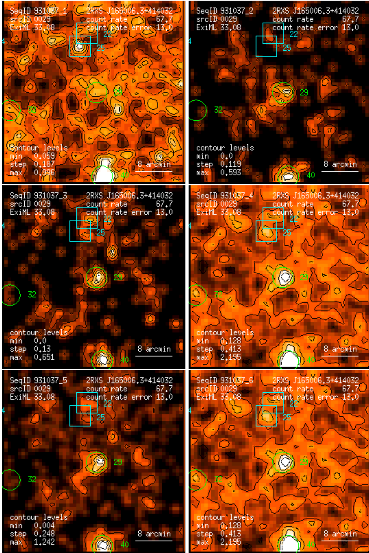
Figure 29: RASS 931037: detection 0029: band rate images, Gaussian filter: (1) PSPC channels 11 – 41, (2) 52 – 90, (3) 91 – 201, (4) 11 – 235, (5) 52 – 201, (6) 11 – 201. Broad band rates in counts/ks. Band rate contour levels in counts/ks/arcmin 2 .
