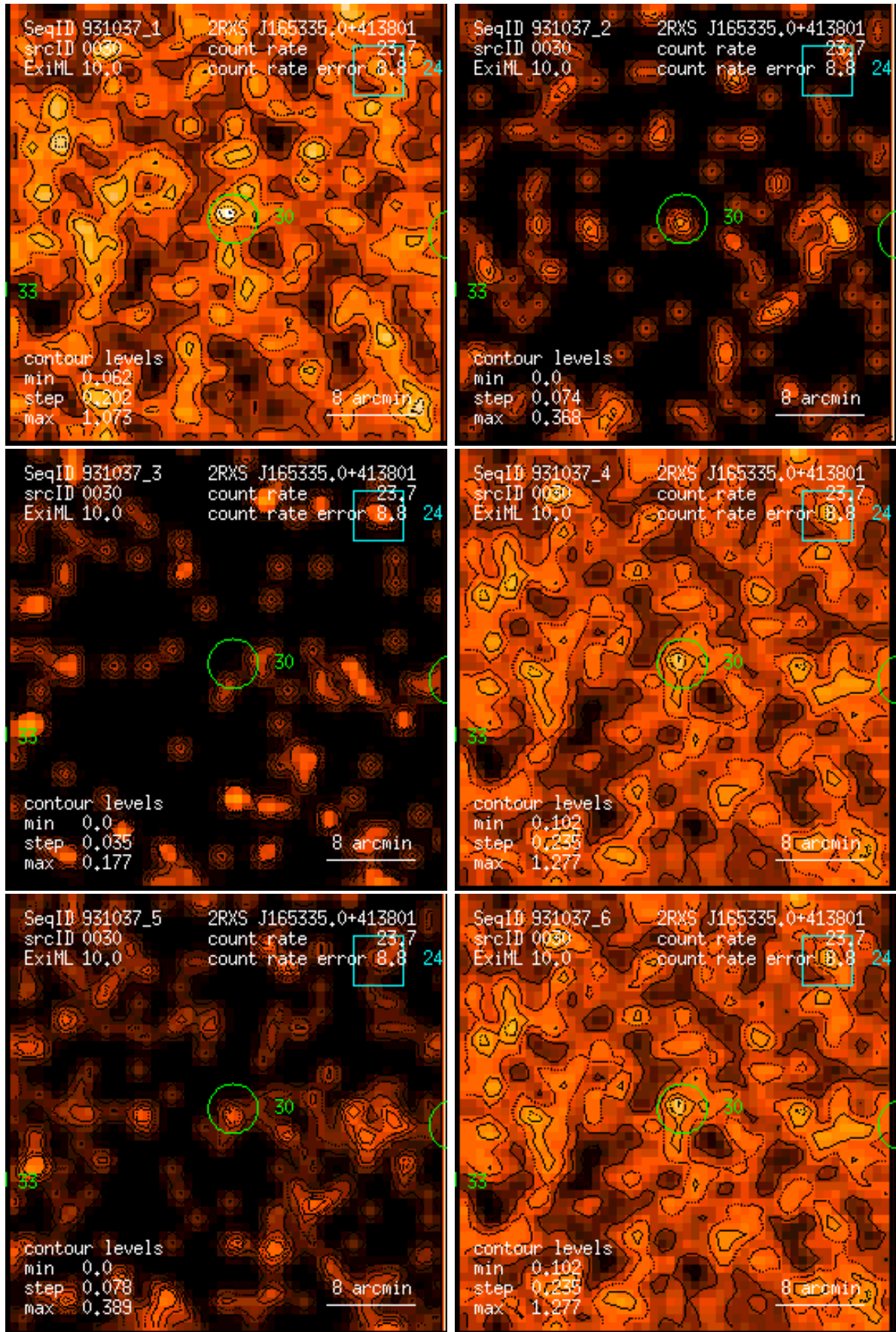
Figure 30: RASS 931037: detection 0030: band rate images, Gaussian filter: (1) PSPC channels 11 – 41, (2) 52 – 90, (3) 91 – 201, (4) 11 – 235, (5) 52 – 201, (6) 11 – 201. Broad band rates in counts/ks. Band rate contour levels in counts/ks/arcmin 2 .
