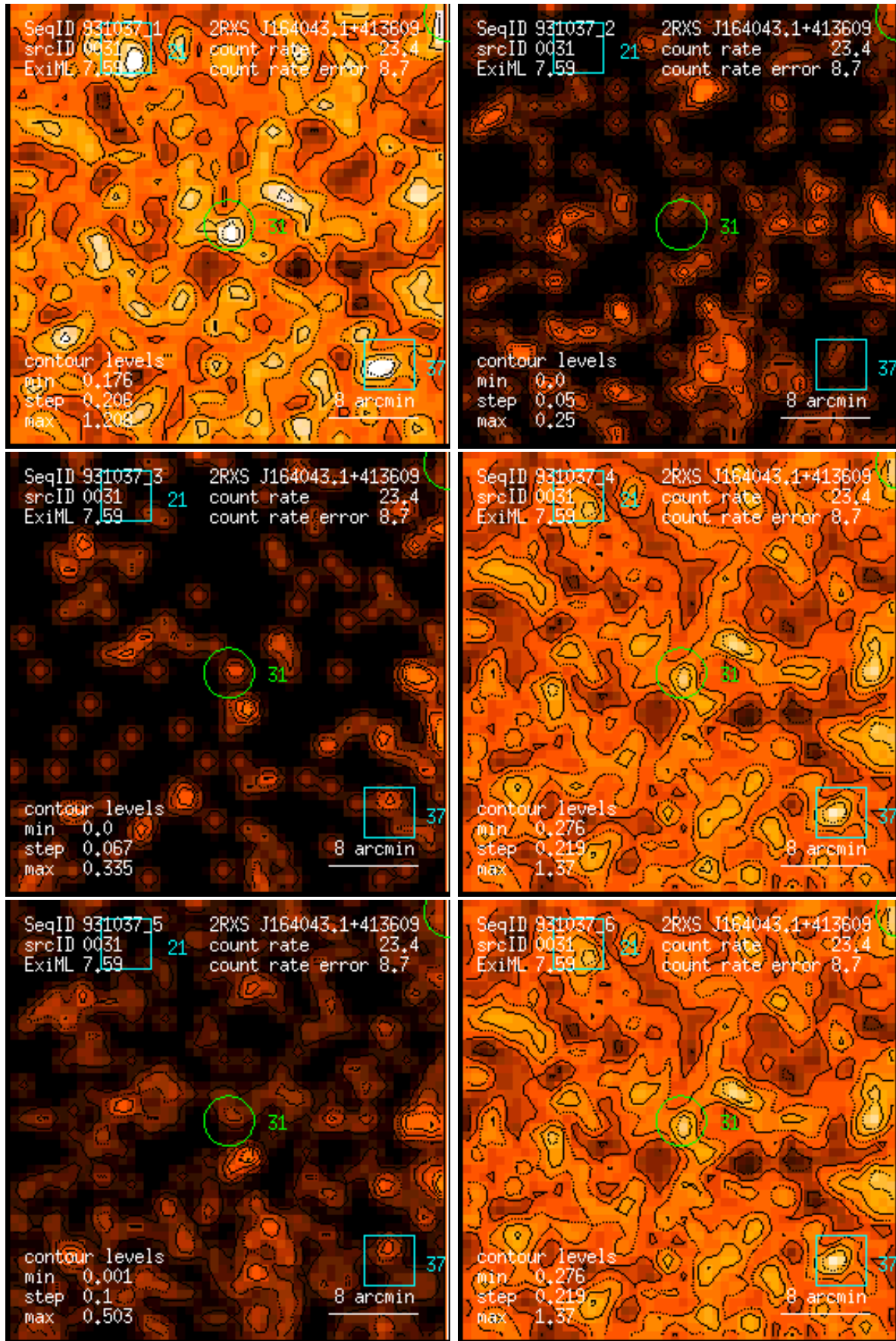
Figure 31: RASS 931037: detection 0031: band rate images, Gaussian filter: (1) PSPC channels 11 – 41, (2) 52 – 90, (3) 91 – 201, (4) 11 – 235, (5) 52 – 201, (6) 11 – 201. Broad band rates in counts/ks. Band rate contour levels in counts/ks/arcmin 2 .
