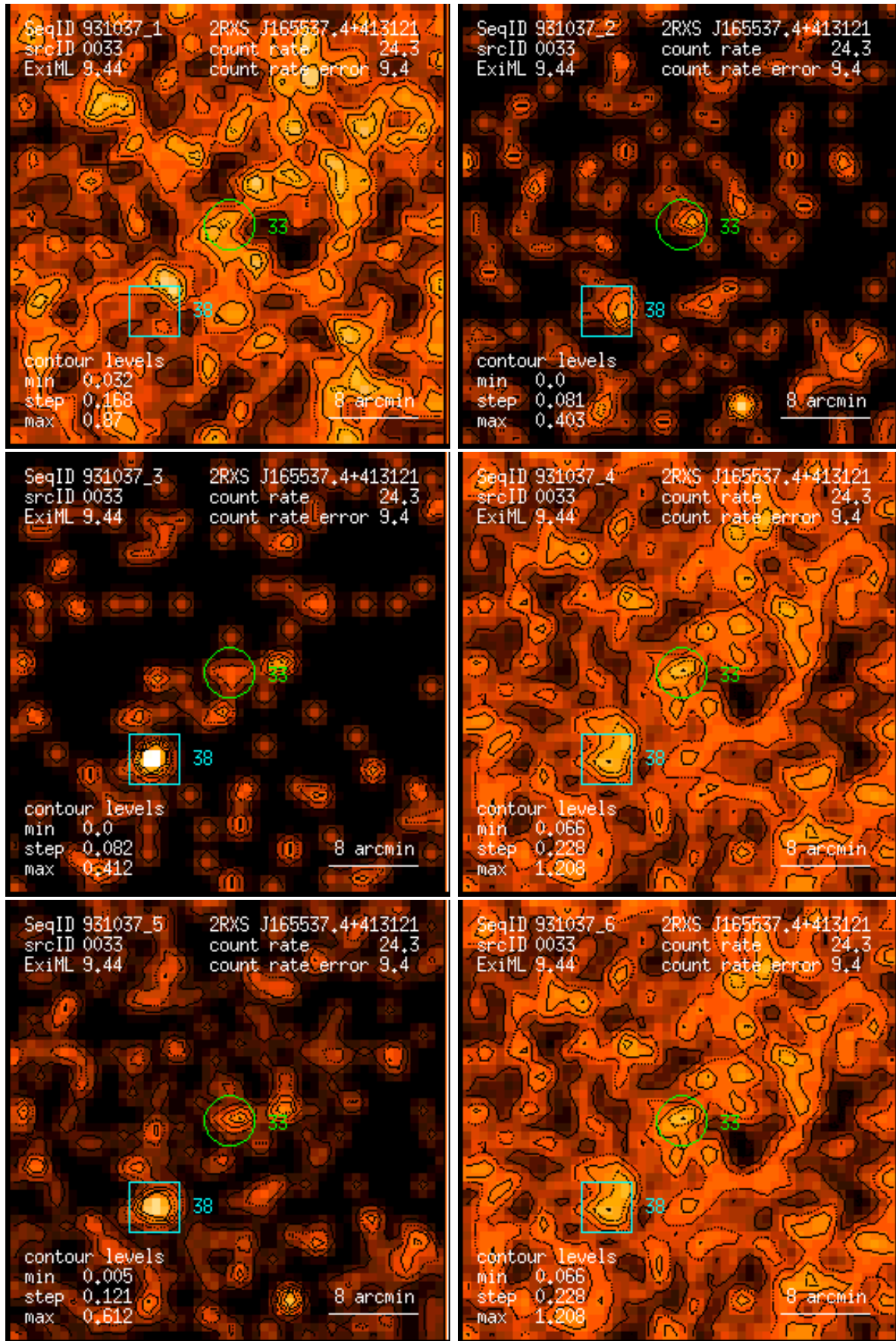
Figure 33: RASS 931037: detection 0033: band rate images, Gaussian filter: (1) PSPC channels 11 – 41, (2) 52 – 90, (3) 91 – 201, (4) 11 – 235, (5) 52 – 201, (6) 11 – 201. Broad band rates in counts/ks. Band rate contour levels in counts/ks/arcmin 2 .
