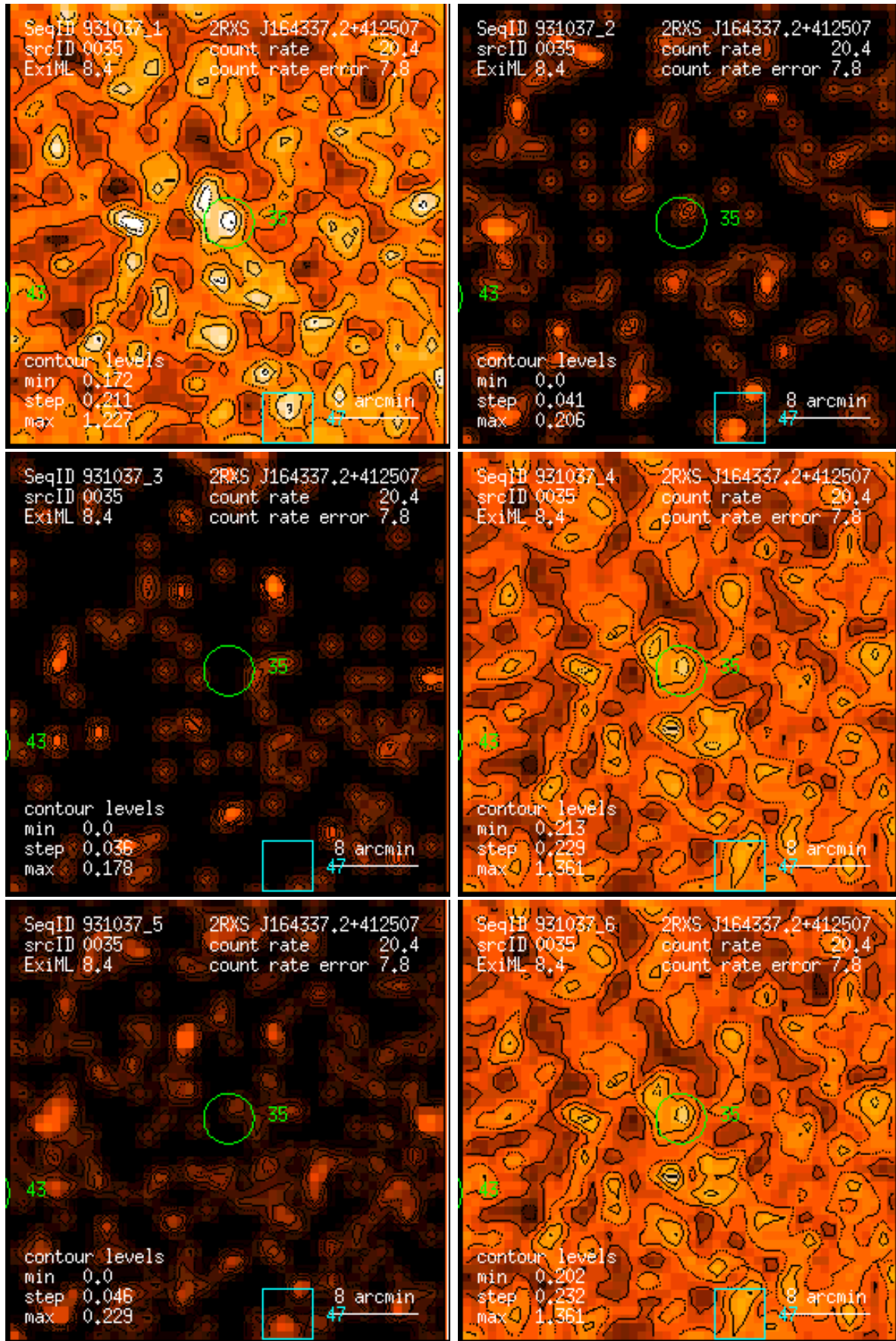
Figure 35: RASS 931037: detection 0035: band rate images, Gaussian filter: (1) PSPC channels 11 – 41, (2) 52 – 90, (3) 91 – 201, (4) 11 – 235, (5) 52 – 201, (6) 11 – 201. Broad band rates in counts/ks. Band rate contour levels in counts/ks/arcmin 2 .
