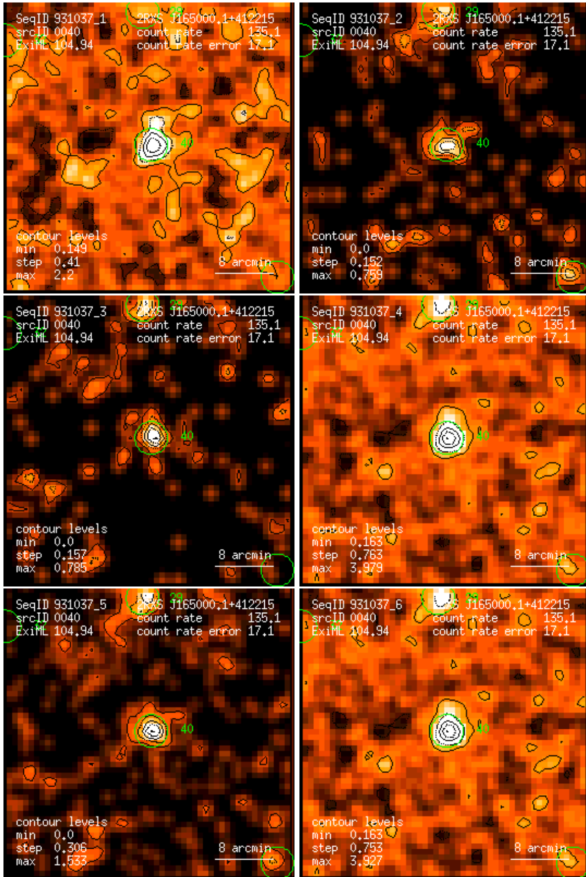
Figure 40: RASS 931037: detection 0040: band rate images, Gaussian filter: (1) PSPC channels 11 – 41, (2) 52 – 90, (3) 91 – 201, (4) 11 – 235, (5) 52 – 201, (6) 11 – 201. Broad band rates in counts/ks. Band rate contour levels in counts/ks/arcmin 2 .
