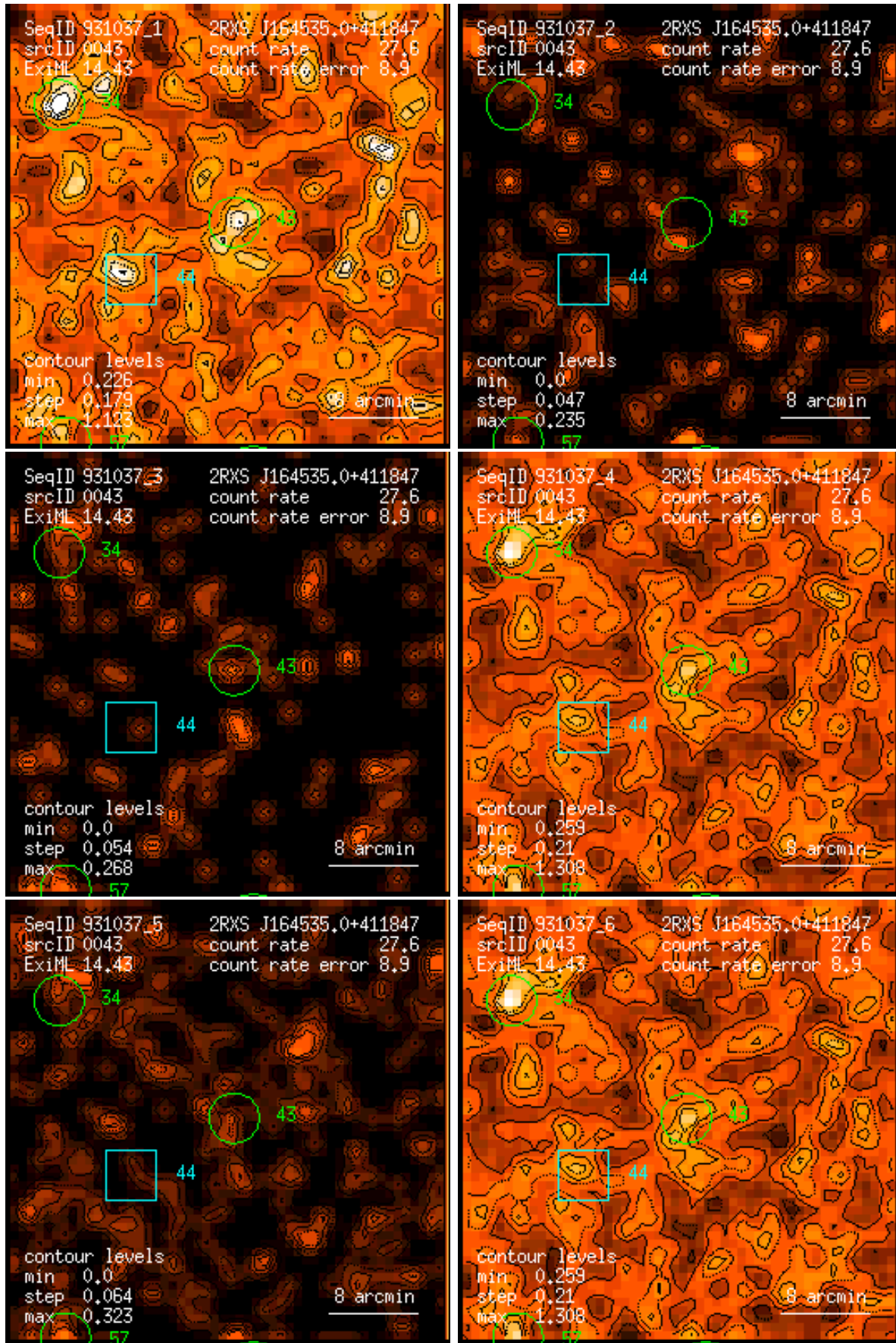
Figure 43: RASS 931037: detection 0043: band rate images, Gaussian filter: (1) PSPC channels 11 – 41, (2) 52 – 90, (3) 91 – 201, (4) 11 – 235, (5) 52 – 201, (6) 11 – 201. Broad band rates in counts/ks. Band rate contour levels in counts/ks/arcmin 2 .
