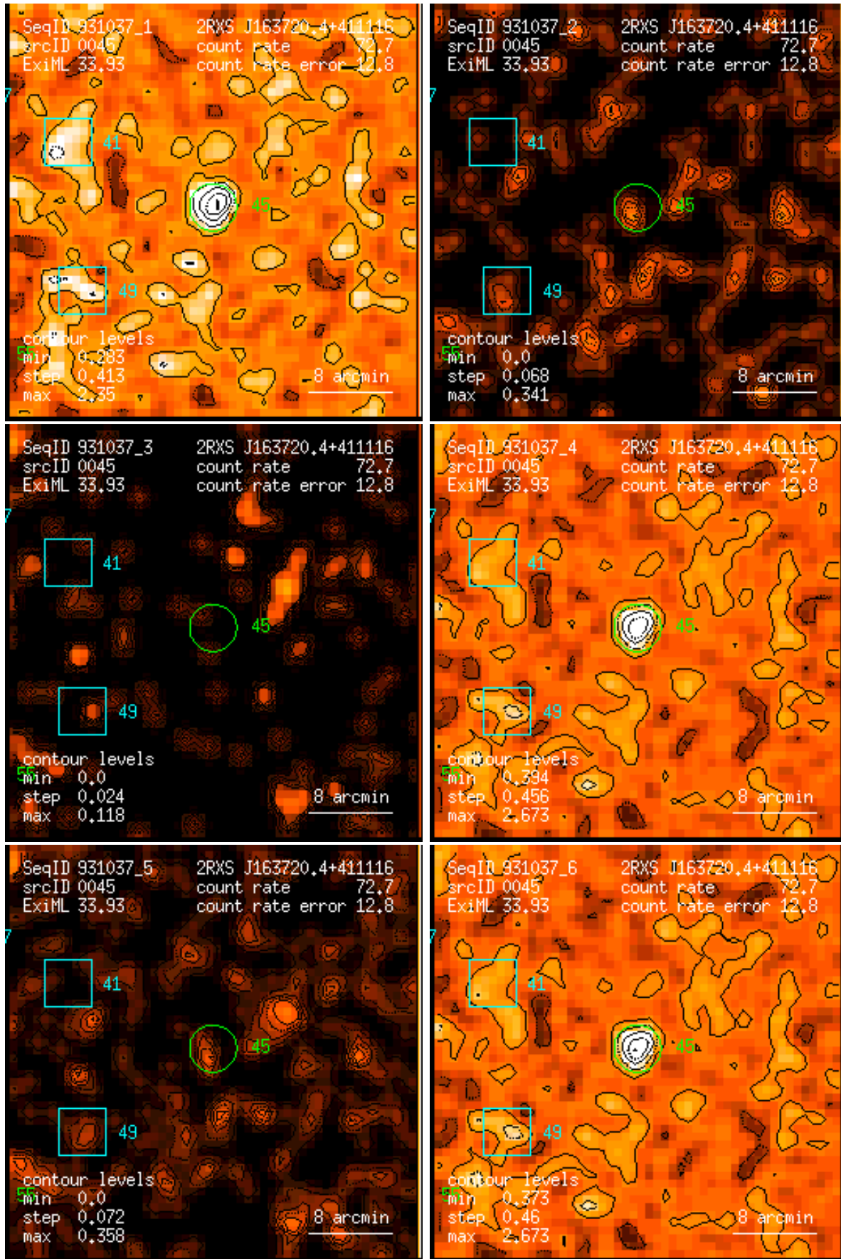
Figure 45: RASS 931037: detection 0045: band rate images, Gaussian filter: (1) PSPC channels 11 – 41, (2) 52 – 90, (3) 91 – 201, (4) 11 – 235, (5) 52 – 201, (6) 11 – 201. Broad band rates in counts/ks. Band rate contour levels in counts/ks/arcmin 2 .
