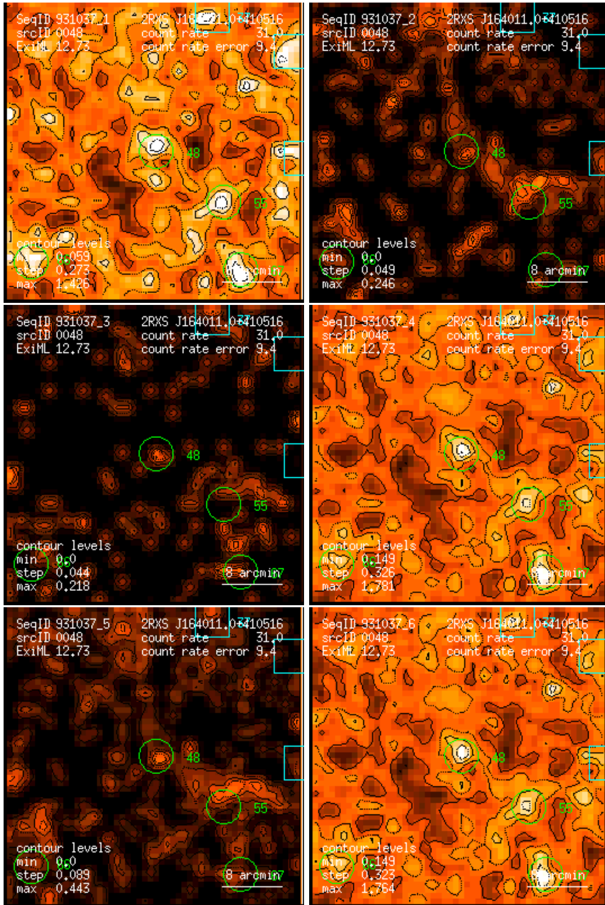
Figure 48: RASS 931037: detection 0048: band rate images, Gaussian filter: (1) PSPC channels 11 – 41, (2) 52 – 90, (3) 91 – 201, (4) 11 – 235, (5) 52 – 201, (6) 11 – 201. Broad band rates in counts/ks. Band rate contour levels in counts/ks/arcmin 2 .
