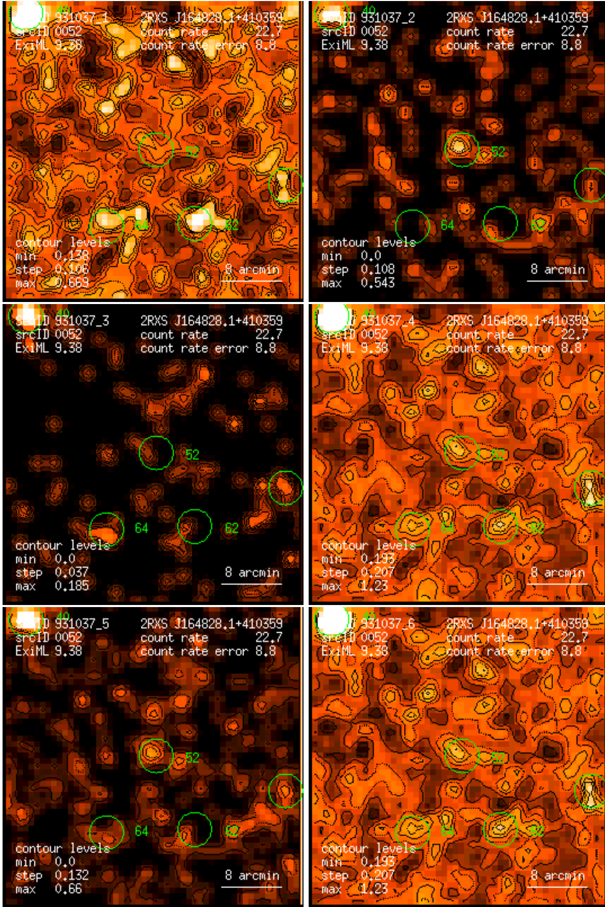
Figure 52: RASS 931037: detection 0052: band rate images, Gaussian filter: (1) PSPC channels 11 – 41, (2) 52 – 90, (3) 91 – 201, (4) 11 – 235, (5) 52 – 201, (6) 11 – 201. Broad band rates in counts/ks. Band rate contour levels in counts/ks/arcmin 2 .
