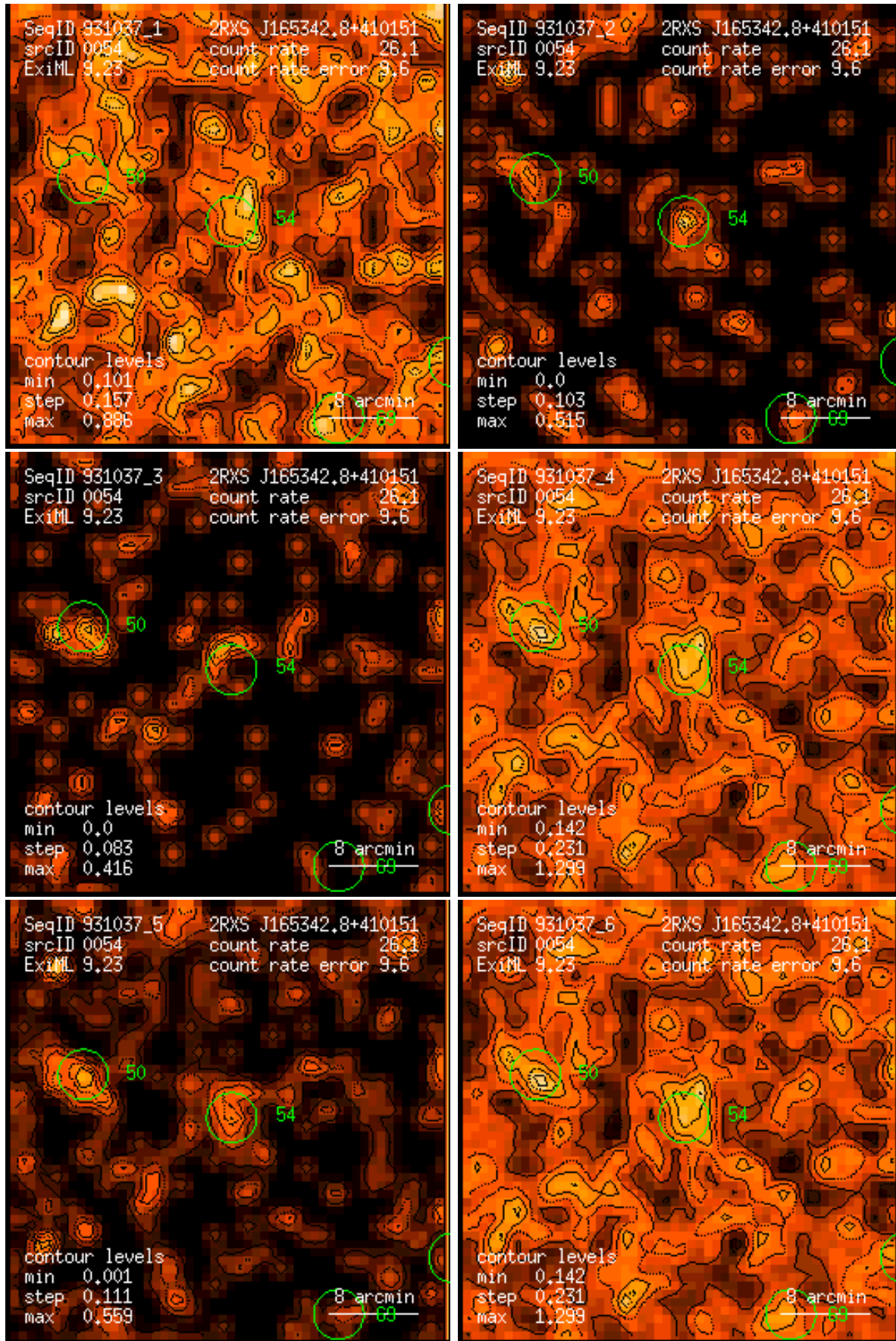
Figure 54: RASS 931037: detection 0054: band rate images, Gaussian filter: (1) PSPC channels 11 – 41, (2) 52 – 90, (3) 91 – 201, (4) 11 – 235, (5) 52 – 201, (6) 11 – 201. Broad band rates in counts/ks. Band rate contour levels in counts/ks/arcmin 2 .
