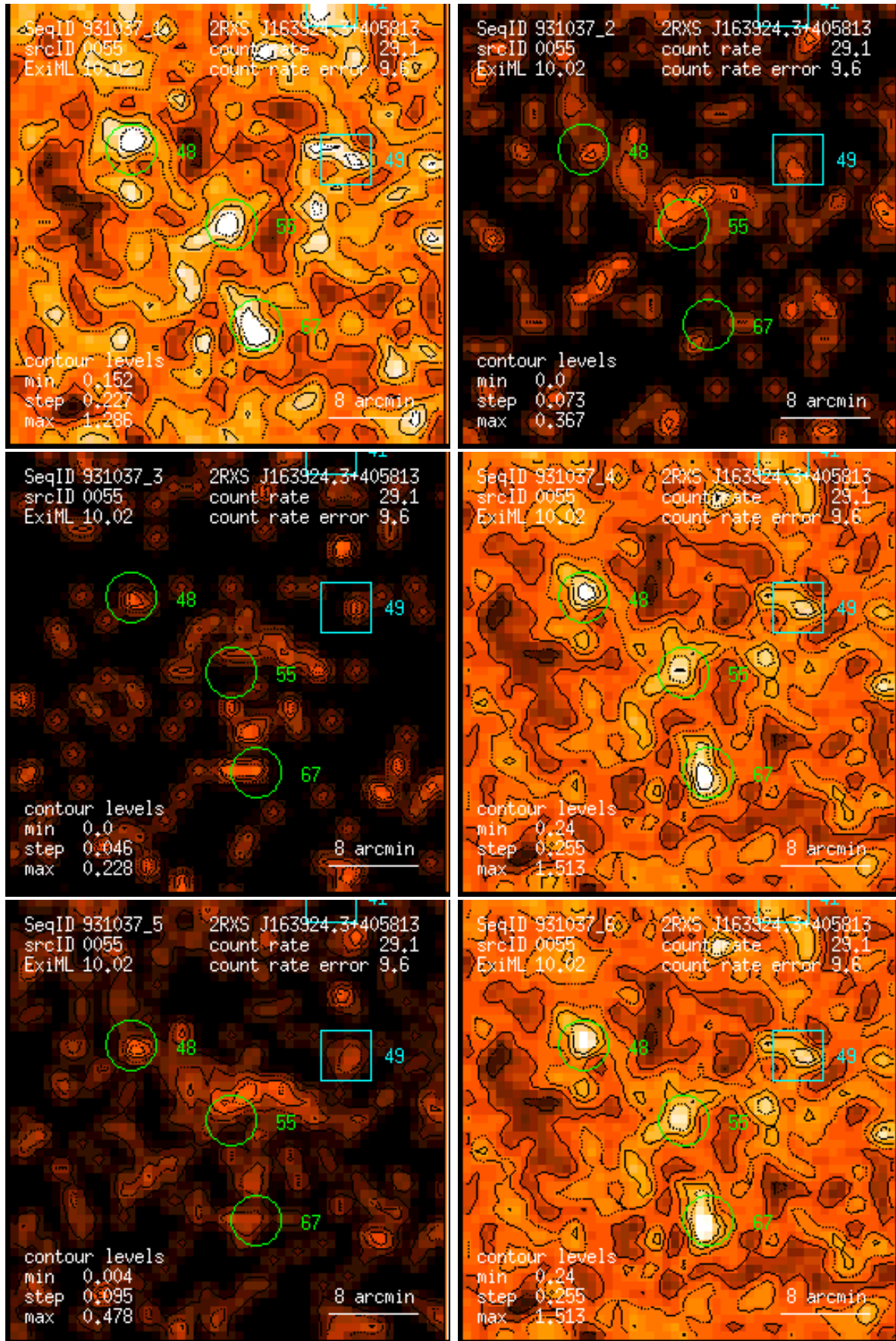
Figure 55: RASS 931037: detection 0055: band rate images, Gaussian filter: (1) PSPC channels 11 – 41, (2) 52 – 90, (3) 91 – 201, (4) 11 – 235, (5) 52 – 201, (6) 11 – 201. Broad band rates in counts/ks. Band rate contour levels in counts/ks/arcmin 2 .
