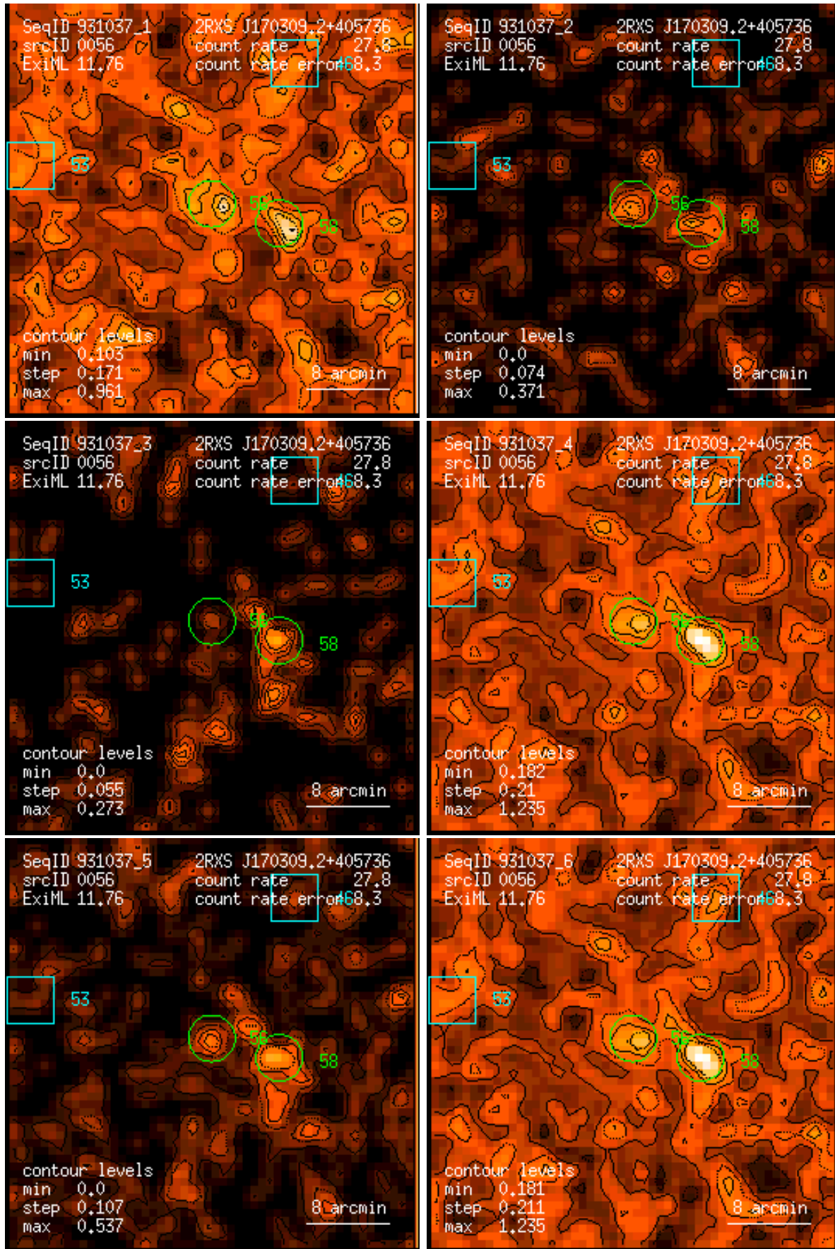
Figure 56: RASS 931037: detection 0056: band rate images, Gaussian filter: (1) PSPC channels 11 – 41, (2) 52 – 90, (3) 91 – 201, (4) 11 – 235, (5) 52 – 201, (6) 11 – 201. Broad band rates in counts/ks. Band rate contour levels in counts/ks/arcmin 2 .
