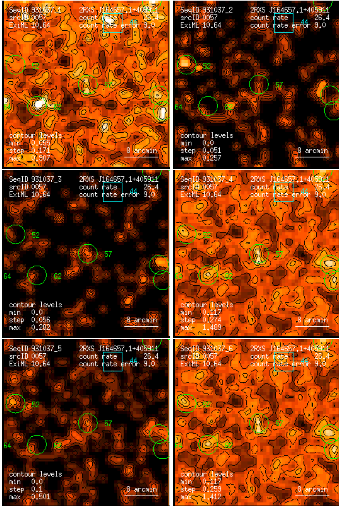
Figure 57: RASS 931037: detection 0057: band rate images, Gaussian filter: (1) PSPC channels 11 – 41, (2) 52 – 90, (3) 91 – 201, (4) 11 – 235, (5) 52 – 201, (6) 11 – 201. Broad band rates in counts/ks. Band rate contour levels in counts/ks/arcmin 2 .
