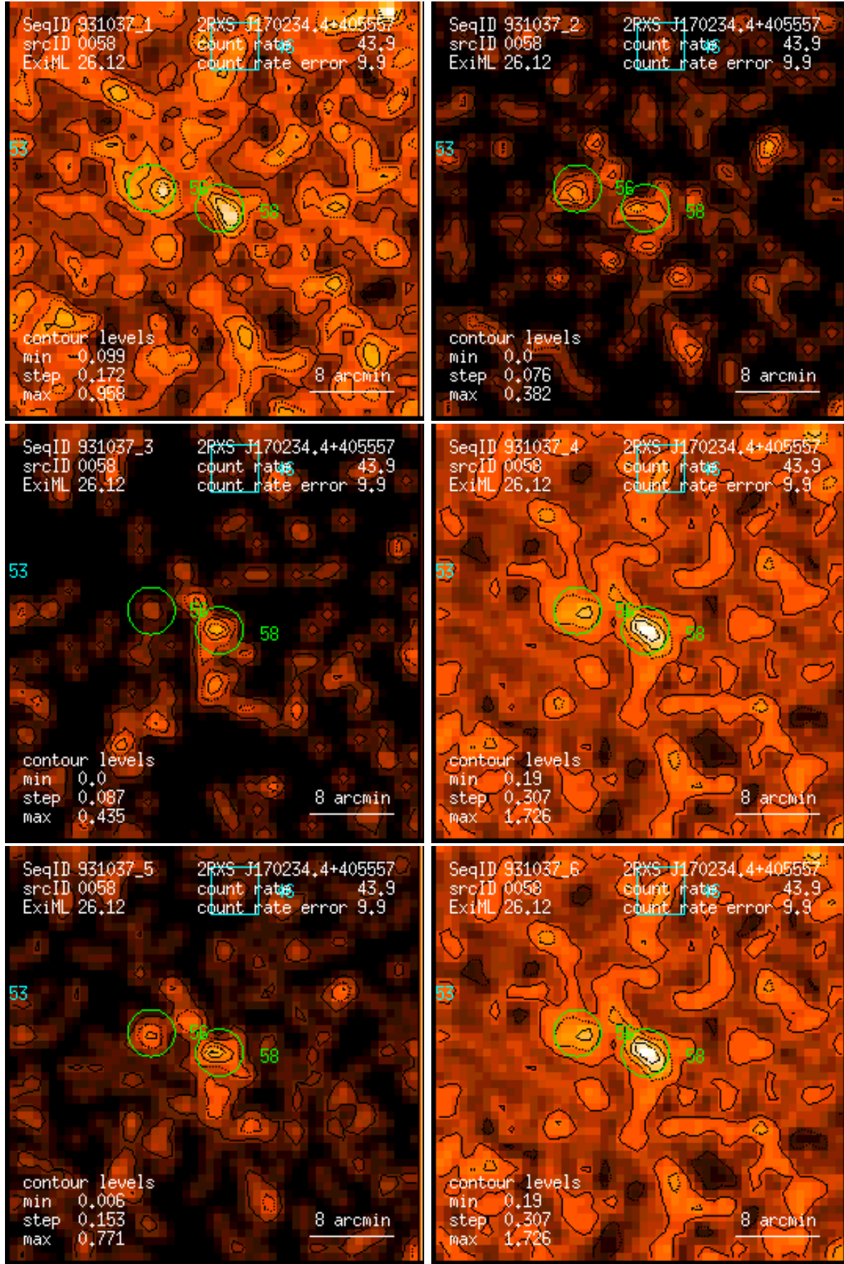
Figure 58: RASS 931037: detection 0058: band rate images, Gaussian filter: (1) PSPC channels 11 – 41, (2) 52 – 90, (3) 91 – 201, (4) 11 – 235, (5) 52 – 201, (6) 11 – 201. Broad band rates in counts/ks. Band rate contour levels in counts/ks/arcmin 2 .
