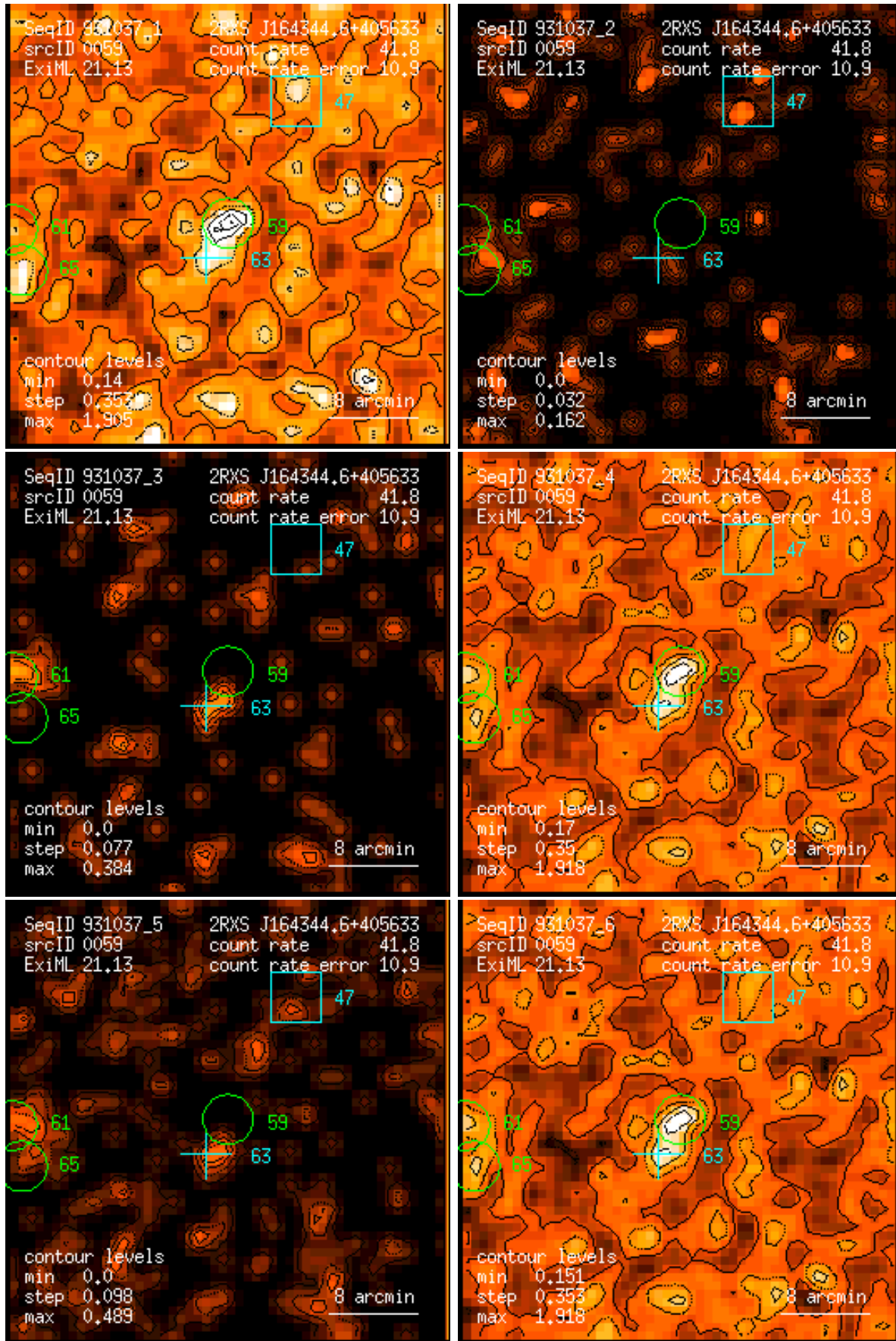
Figure 59: RASS 931037: detection 0059: band rate images, Gaussian filter: (1) PSPC channels 11 – 41, (2) 52 – 90, (3) 91 – 201, (4) 11 – 235, (5) 52 – 201, (6) 11 – 201. Broad band rates in counts/ks. Band rate contour levels in counts/ks/arcmin 2 .
