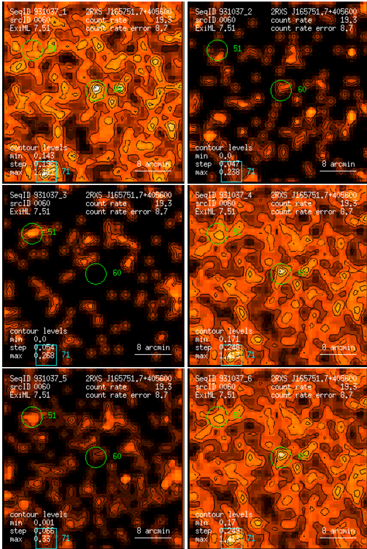
Figure 60: RASS 931037: detection 0060: band rate images, Gaussian filter: (1) PSPC channels 11 – 41, (2) 52 – 90, (3) 91 – 201, (4) 11 – 235, (5) 52 – 201, (6) 11 – 201. Broad band rates in counts/ks. Band rate contour levels in counts/ks/arcmin 2 .
