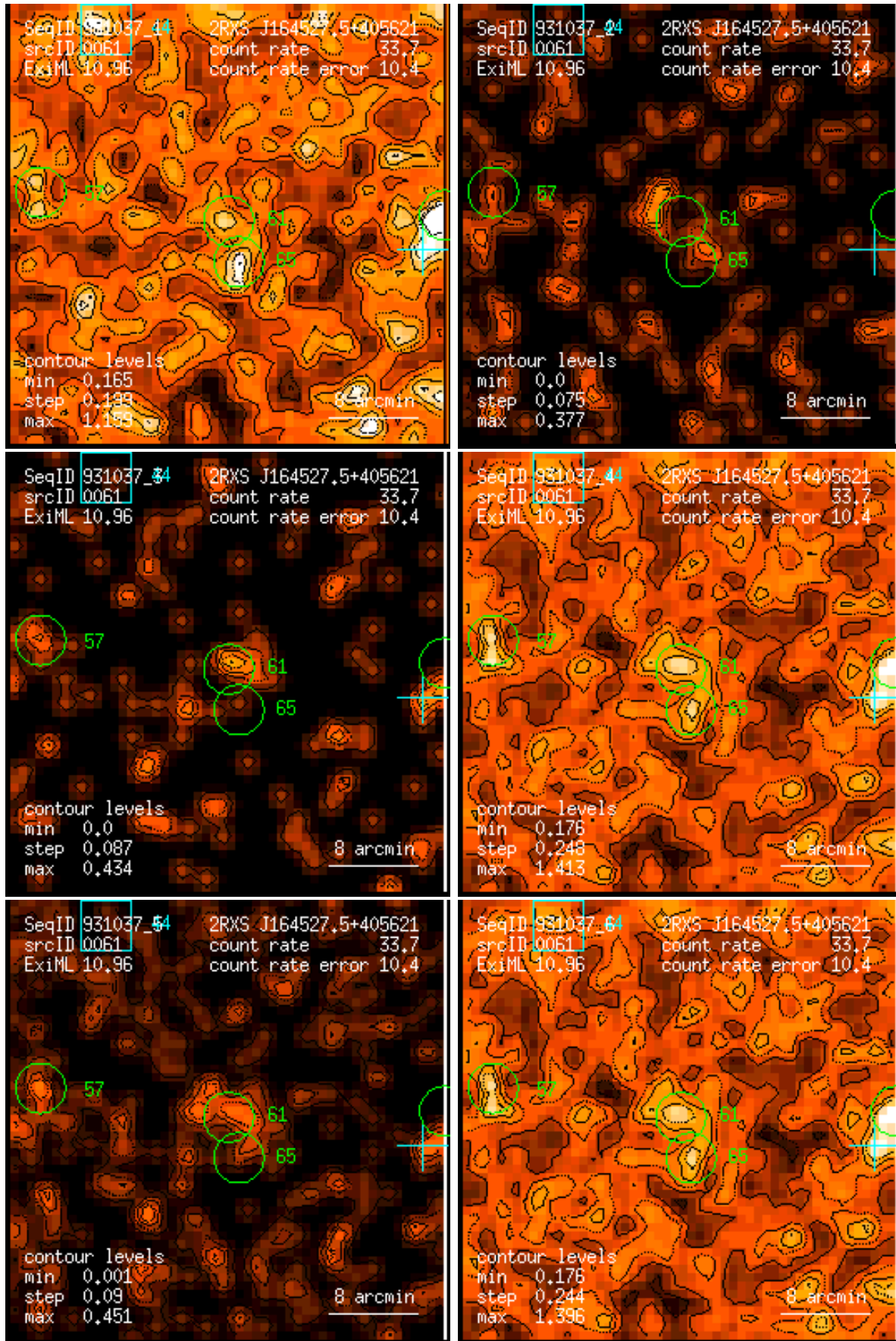
Figure 61: RASS 931037: detection 0061: band rate images, Gaussian filter: (1) PSPC channels 11 – 41, (2) 52 – 90, (3) 91 – 201, (4) 11 – 235, (5) 52 – 201, (6) 11 – 201. Broad band rates in counts/ks. Band rate contour levels in counts/ks/arcmin 2 .
