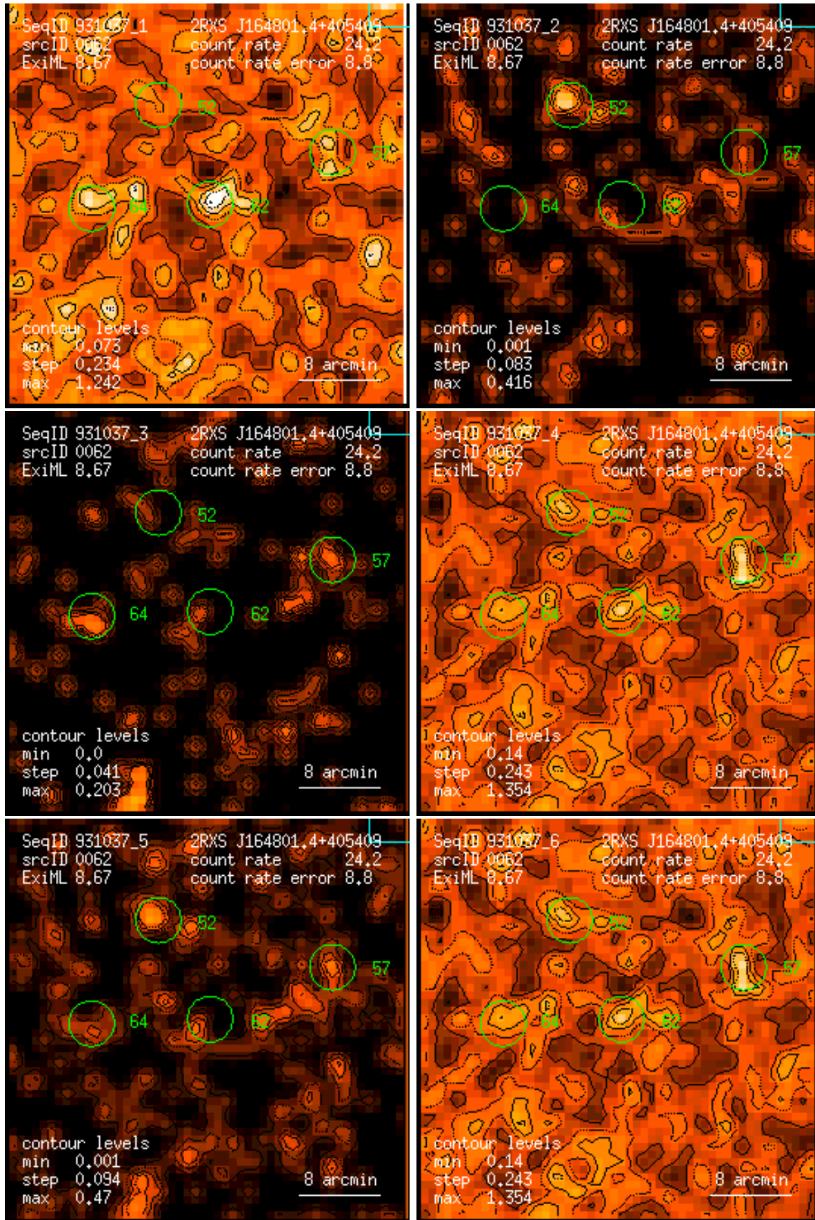
Figure 62: RASS 931037: detection 0062: band rate images, Gaussian filter: (1) PSPC channels 11 – 41, (2) 52 – 90, (3) 91 – 201, (4) 11 – 235, (5) 52 – 201, (6) 11 – 201. Broad band rates in counts/ks. Band rate contour levels in counts/ks/arcmin 2 .
