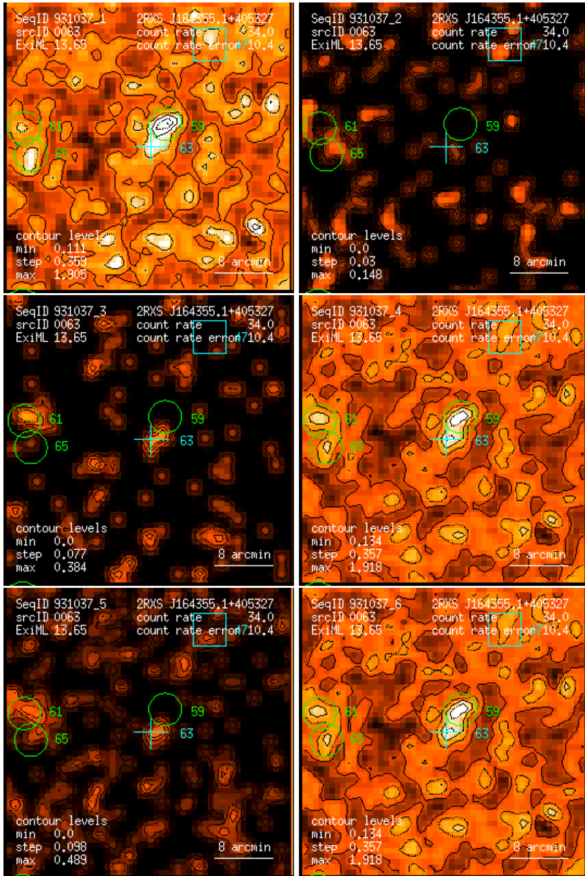
Figure 63: RASS 931037: detection 0063: band rate images, Gaussian filter: (1) PSPC channels 11 – 41, (2) 52 – 90, (3) 91 – 201, (4) 11 – 235, (5) 52 – 201, (6) 11 – 201. Broad band rates in counts/ks. Band rate contour levels in counts/ks/arcmin 2 .
