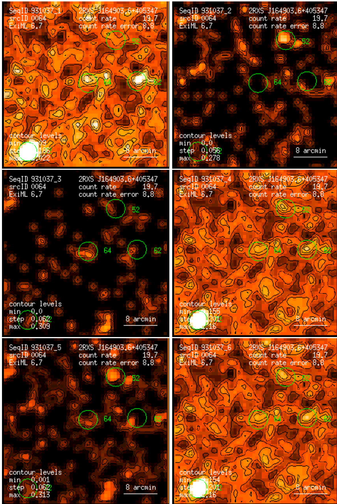
Figure 64: RASS 931037: detection 0064: band rate images, Gaussian filter: (1) PSPC channels 11 – 41, (2) 52 – 90, (3) 91 – 201, (4) 11 – 235, (5) 52 – 201, (6) 11 – 201. Broad band rates in counts/ks. Band rate contour levels in counts/ks/arcmin 2 .
