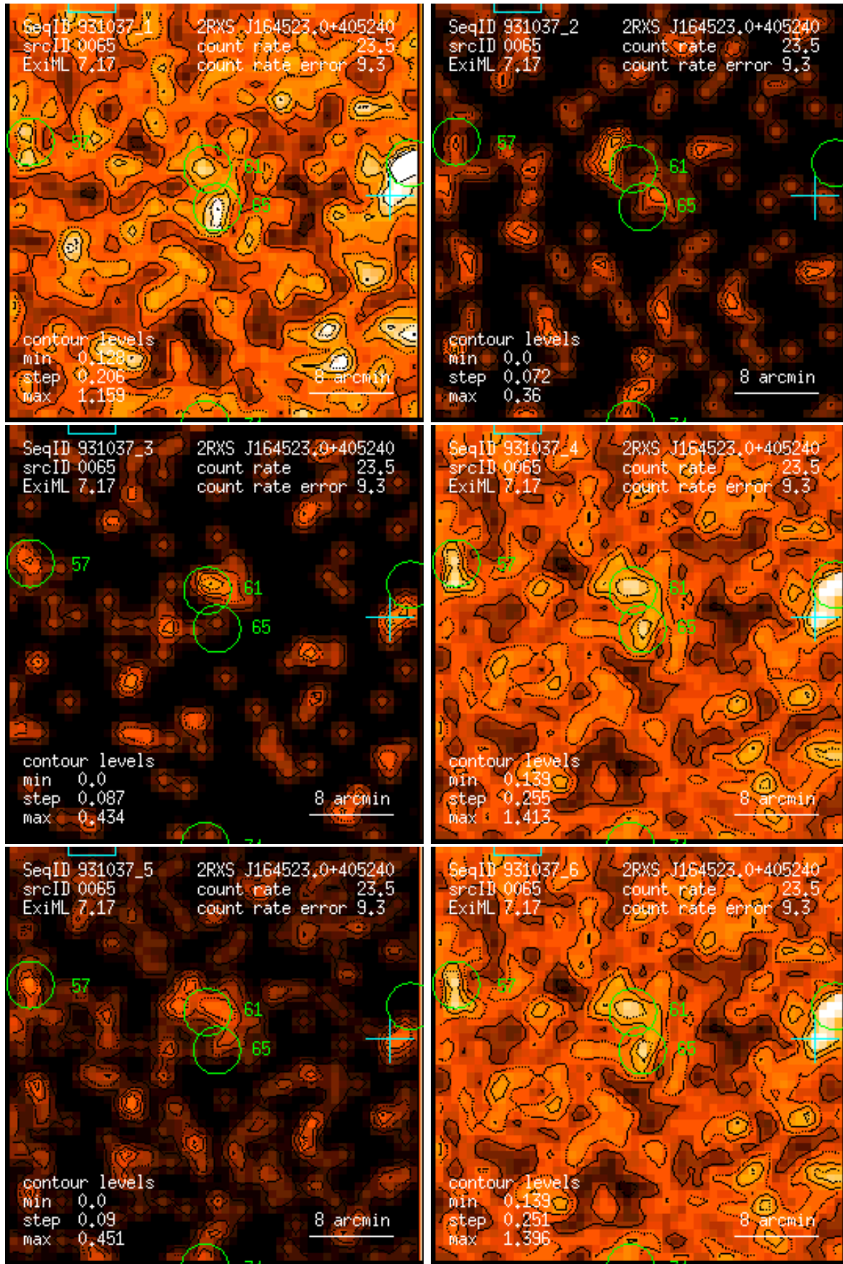
Figure 65: RASS 931037: detection 0065: band rate images, Gaussian filter: (1) PSPC channels 11 – 41, (2) 52 – 90, (3) 91 – 201, (4) 11 – 235, (5) 52 – 201, (6) 11 – 201. Broad band rates in counts/ks. Band rate contour levels in counts/ks/arcmin 2 .
