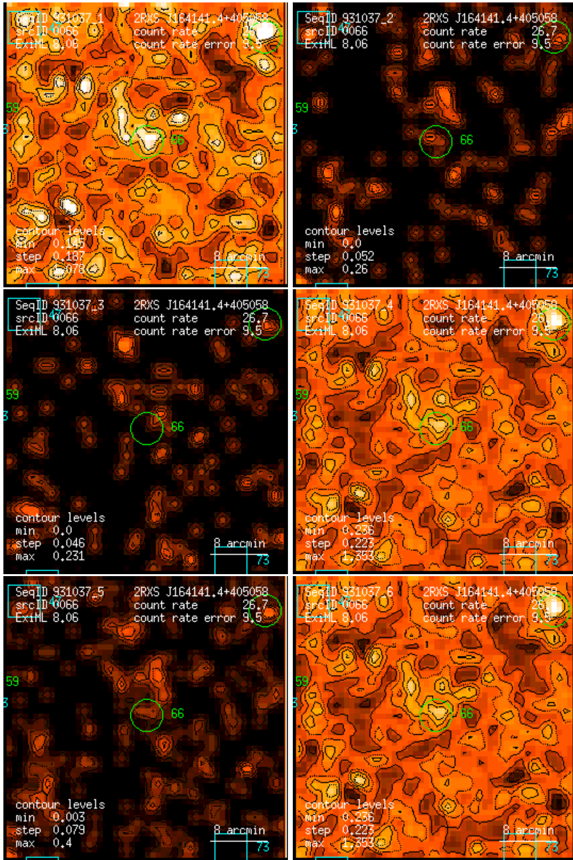
Figure 66: RASS 931037: detection 0066: band rate images, Gaussian filter: (1) PSPC channels 11 – 41, (2) 52 – 90, (3) 91 – 201, (4) 11 – 235, (5) 52 – 201, (6) 11 – 201. Broad band rates in counts/ks. Band rate contour levels in counts/ks/arcmin 2 .
