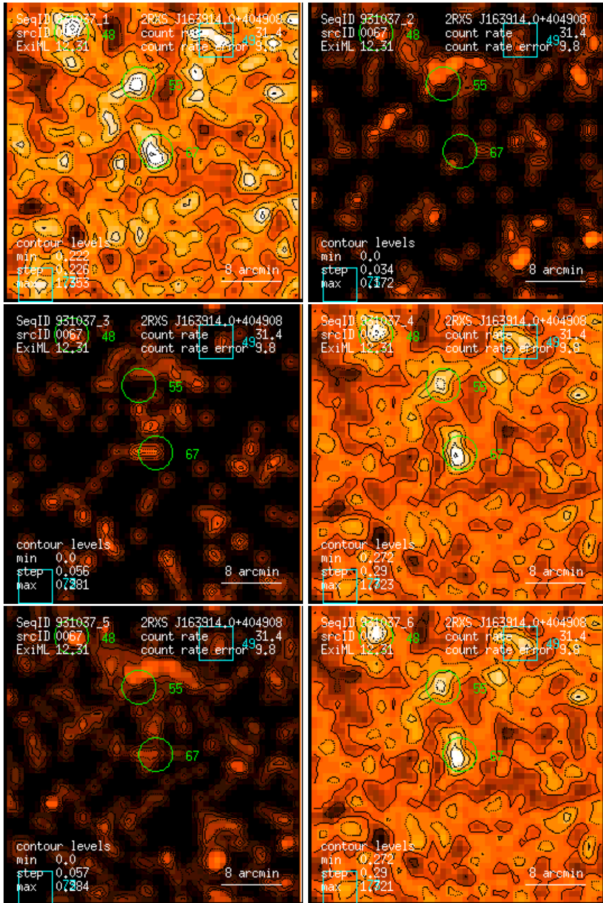
Figure 67: RASS 931037: detection 0067: band rate images, Gaussian filter: (1) PSPC channels 11 – 41, (2) 52 – 90, (3) 91 – 201, (4) 11 – 235, (5) 52 – 201, (6) 11 – 201. Broad band rates in counts/ks. Band rate contour levels in counts/ks/arcmin 2 .
