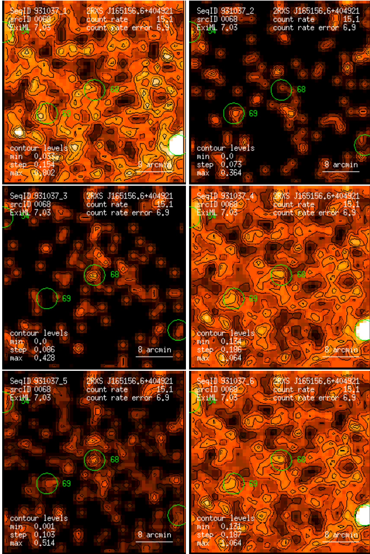
Figure 68: RASS 931037: detection 0068: band rate images, Gaussian filter: (1) PSPC channels 11 – 41, (2) 52 – 90, (3) 91 – 201, (4) 11 – 235, (5) 52 – 201, (6) 11 – 201. Broad band rates in counts/ks. Band rate contour levels in counts/ks/arcmin 2 .
