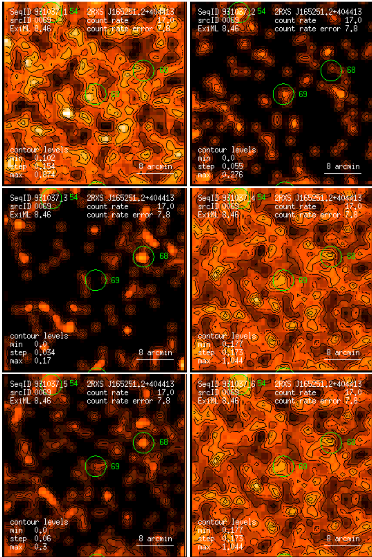
Figure 69: RASS 931037: detection 0069: band rate images, Gaussian filter: (1) PSPC channels 11 – 41, (2) 52 – 90, (3) 91 – 201, (4) 11 – 235, (5) 52 – 201, (6) 11 – 201. Broad band rates in counts/ks. Band rate contour levels in counts/ks/arcmin 2 .
