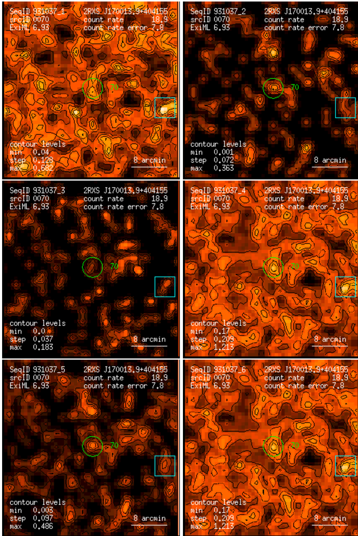
Figure 70: RASS 931037: detection 0070: band rate images, Gaussian filter: (1) PSPC channels 11 – 41, (2) 52 – 90, (3) 91 – 201, (4) 11 – 235, (5) 52 – 201, (6) 11 – 201. Broad band rates in counts/ks. Band rate contour levels in counts/ks/arcmin 2 .
