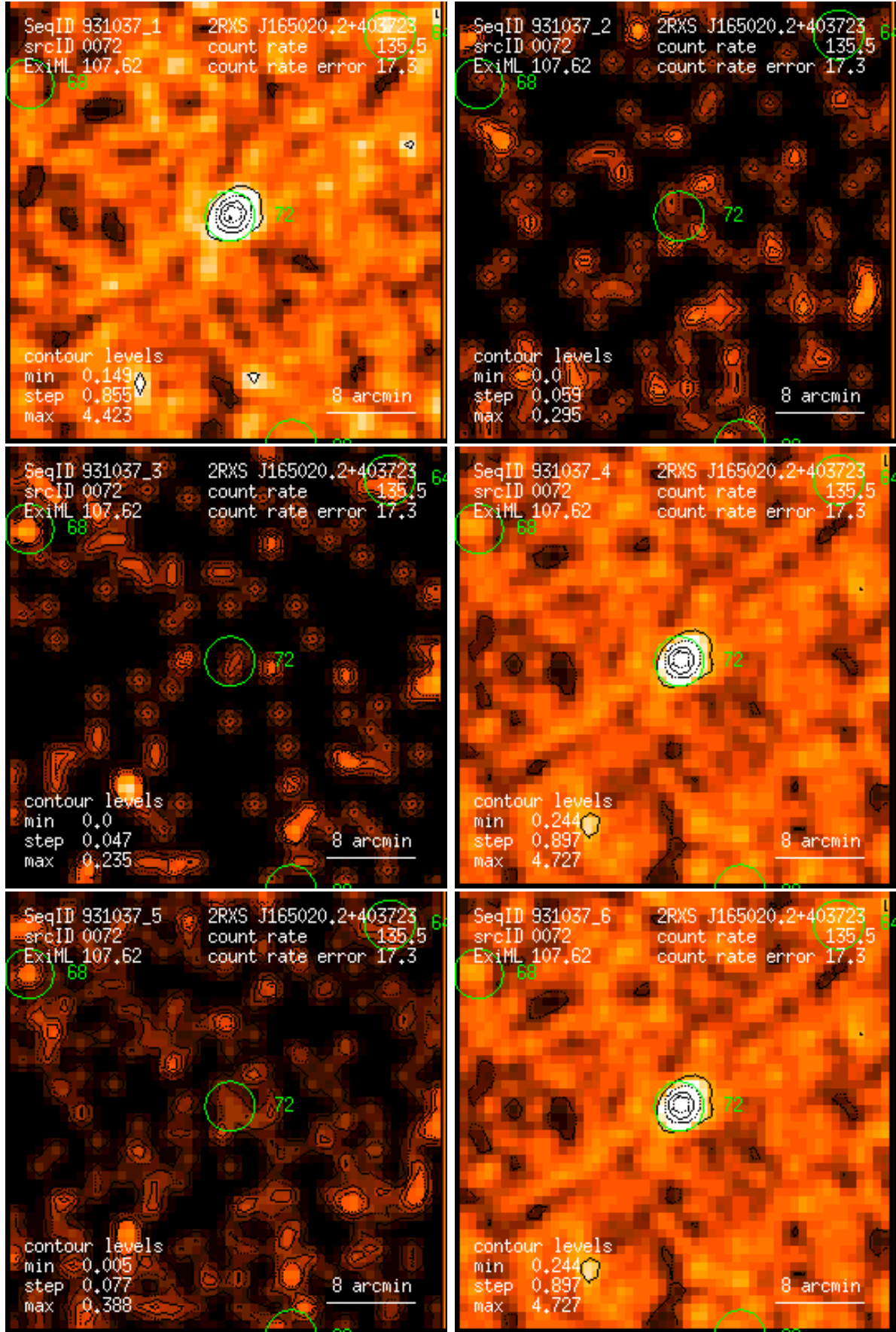
Figure 72: RASS 931037: detection 0072: band rate images, Gaussian filter: (1) PSPC channels 11 – 41, (2) 52 – 90, (3) 91 – 201, (4) 11 – 235, (5) 52 – 201, (6) 11 – 201. Broad band rates in counts/ks. Band rate contour levels in counts/ks/arcmin 2 .
