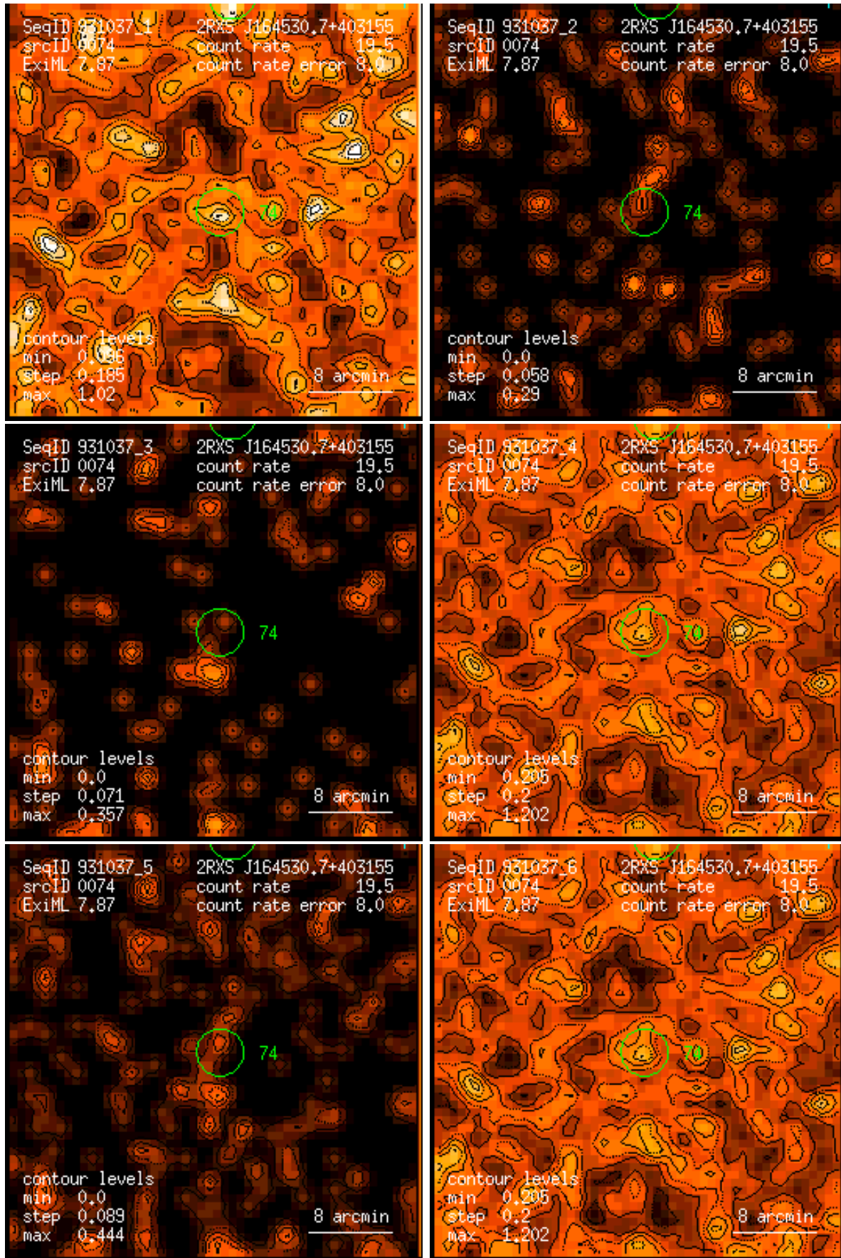
Figure 74: RASS 931037: detection 0074: band rate images, Gaussian filter: (1) PSPC channels 11 – 41, (2) 52 – 90, (3) 91 – 201, (4) 11 – 235, (5) 52 – 201, (6) 11 – 201. Broad band rates in counts/ks. Band rate contour levels in counts/ks/arcmin 2 .
