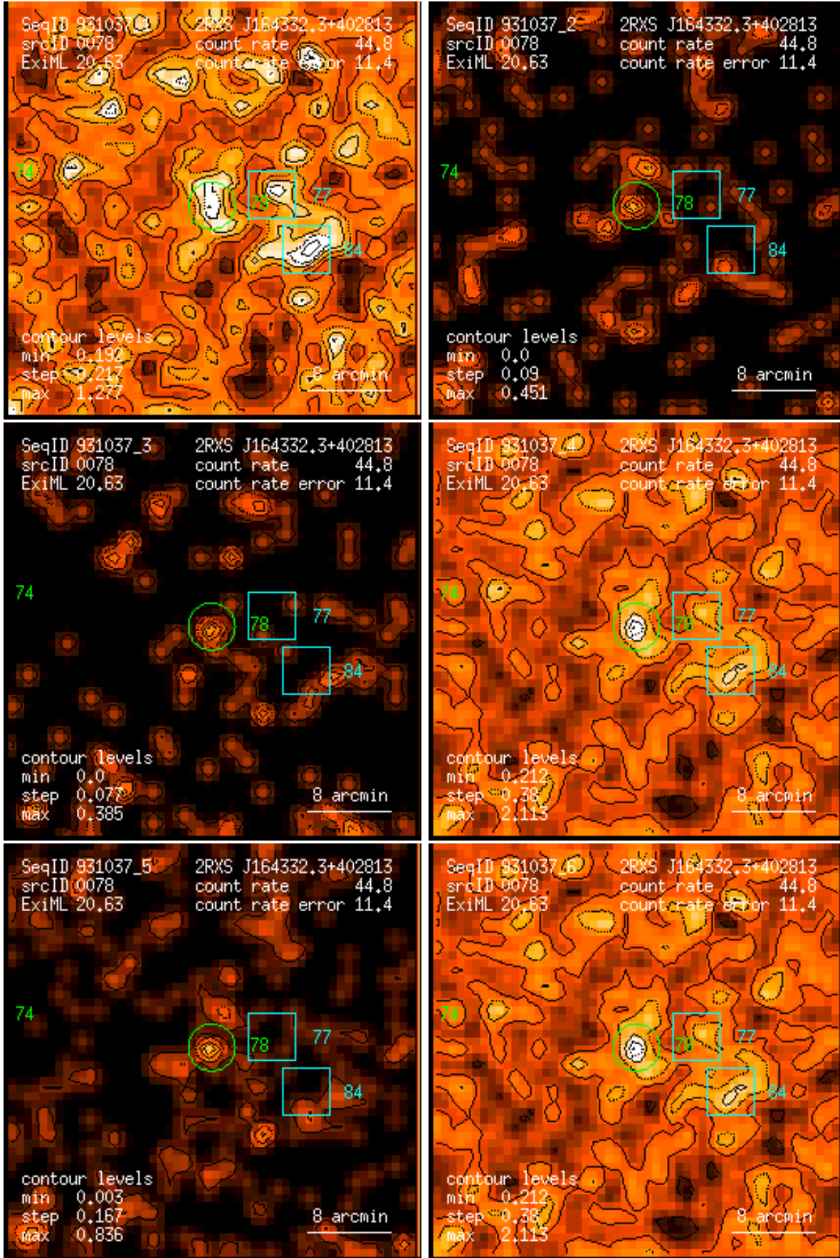
Figure 78: RASS 931037: detection 0078: band rate images, Gaussian filter: (1) PSPC channels 11 – 41, (2) 52 – 90, (3) 91 – 201, (4) 11 – 235, (5) 52 – 201, (6) 11 – 201. Broad band rates in counts/ks. Band rate contour levels in counts/ks/arcmin 2 .
