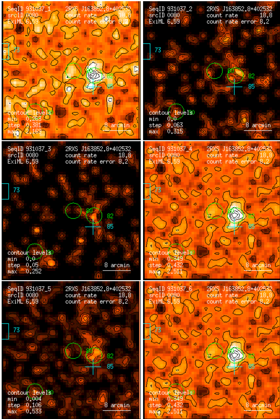
Figure 80: RASS 931037: detection 0080: band rate images, Gaussian filter: (1) PSPC channels 11 – 41, (2) 52 – 90, (3) 91 – 201, (4) 11 – 235, (5) 52 – 201, (6) 11 – 201. Broad band rates in counts/ks. Band rate contour levels in counts/ks/arcmin 2 .
