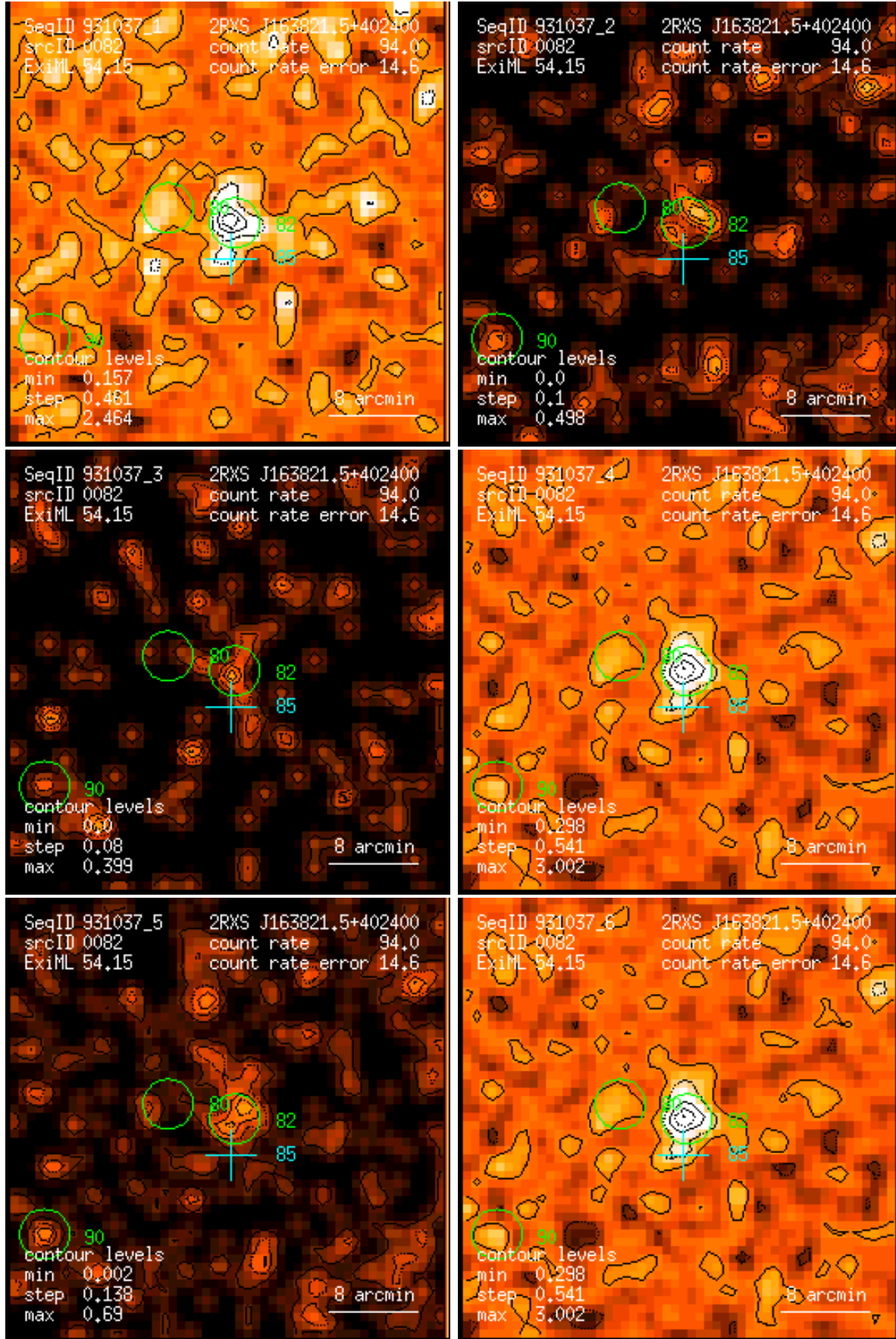
Figure 82: RASS 931037: detection 0082: band rate images, Gaussian filter: (1) PSPC channels 11 – 41, (2) 52 – 90, (3) 91 – 201, (4) 11 – 235, (5) 52 – 201, (6) 11 – 201. Broad band rates in counts/ks. Band rate contour levels in counts/ks/arcmin 2 .
