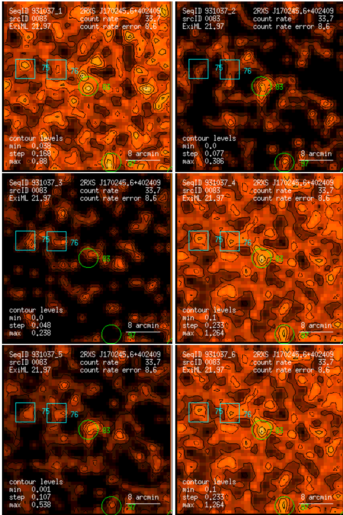
Figure 83: RASS 931037: detection 0083: band rate images, Gaussian filter: (1) PSPC channels 11 – 41, (2) 52 – 90, (3) 91 – 201, (4) 11 – 235, (5) 52 – 201, (6) 11 – 201. Broad band rates in counts/ks. Band rate contour levels in counts/ks/arcmin 2 .
