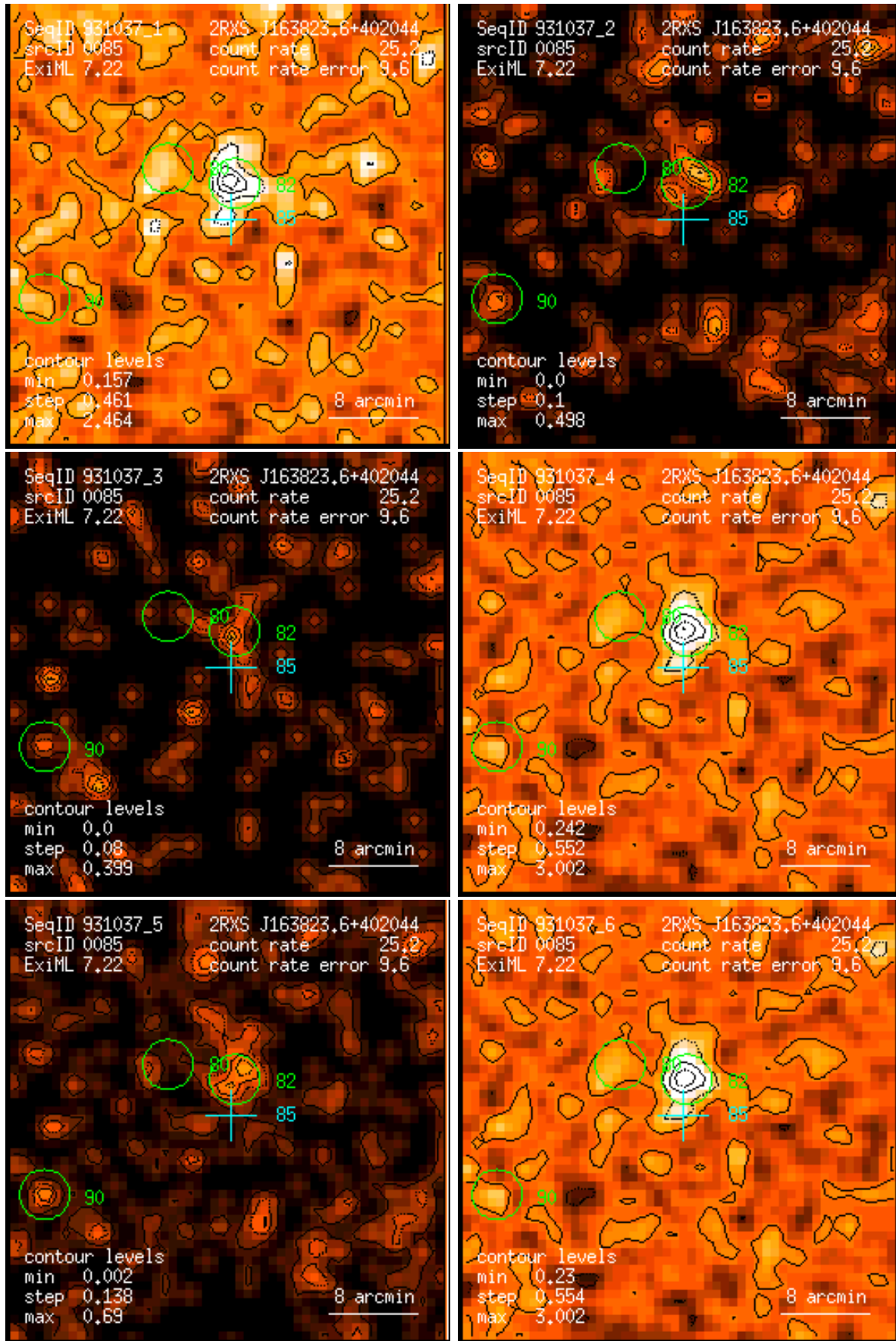
Figure 85: RASS 931037: detection 0085: band rate images, Gaussian filter: (1) PSPC channels 11 – 41, (2) 52 – 90, (3) 91 – 201, (4) 11 – 235, (5) 52 – 201, (6) 11 – 201. Broad band rates in counts/ks. Band rate contour levels in counts/ks/arcmin 2 .
