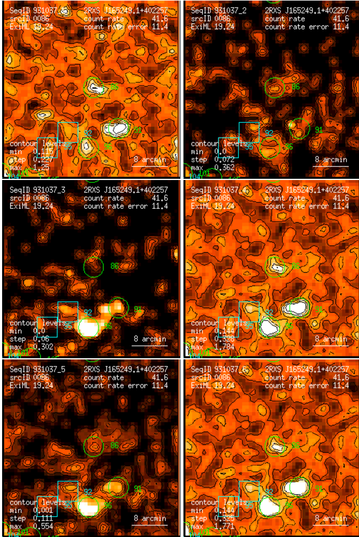
Figure 86: RASS 931037: detection 0086: band rate images, Gaussian filter: (1) PSPC channels 11 – 41, (2) 52 – 90, (3) 91 – 201, (4) 11 – 235, (5) 52 – 201, (6) 11 – 201. Broad band rates in counts/ks. Band rate contour levels in counts/ks/arcmin 2 .
