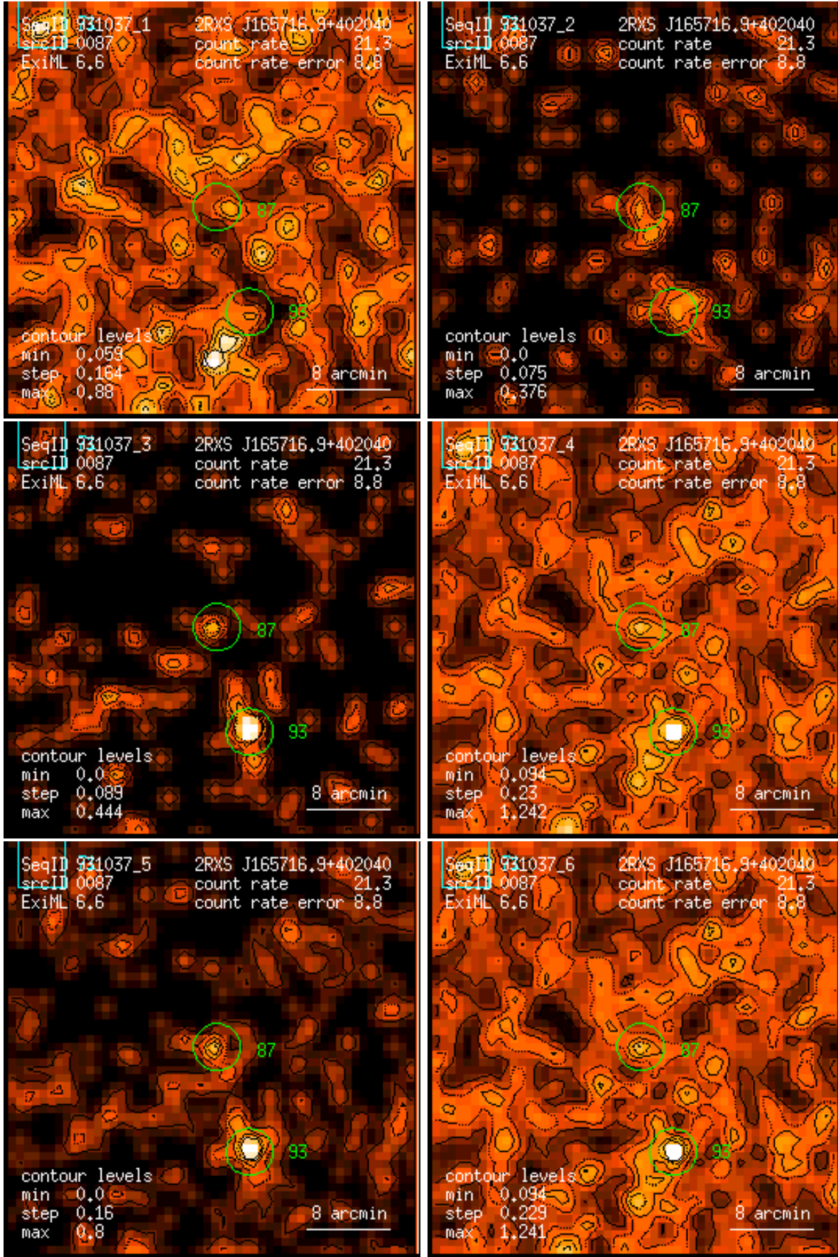
Figure 87: RASS 931037: detection 0087: band rate images, Gaussian filter: (1) PSPC channels 11 – 41, (2) 52 – 90, (3) 91 – 201, (4) 11 – 235, (5) 52 – 201, (6) 11 – 201. Broad band rates in counts/ks. Band rate contour levels in counts/ks/arcmin 2 .
