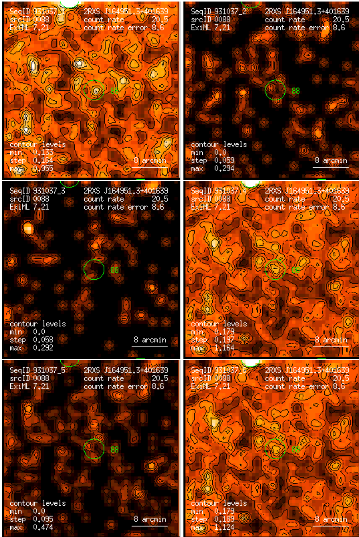
Figure 88: RASS 931037: detection 0088: band rate images, Gaussian filter: (1) PSPC channels 11 – 41, (2) 52 – 90, (3) 91 – 201, (4) 11 – 235, (5) 52 – 201, (6) 11 – 201. Broad band rates in counts/ks. Band rate contour levels in counts/ks/arcmin 2 .
