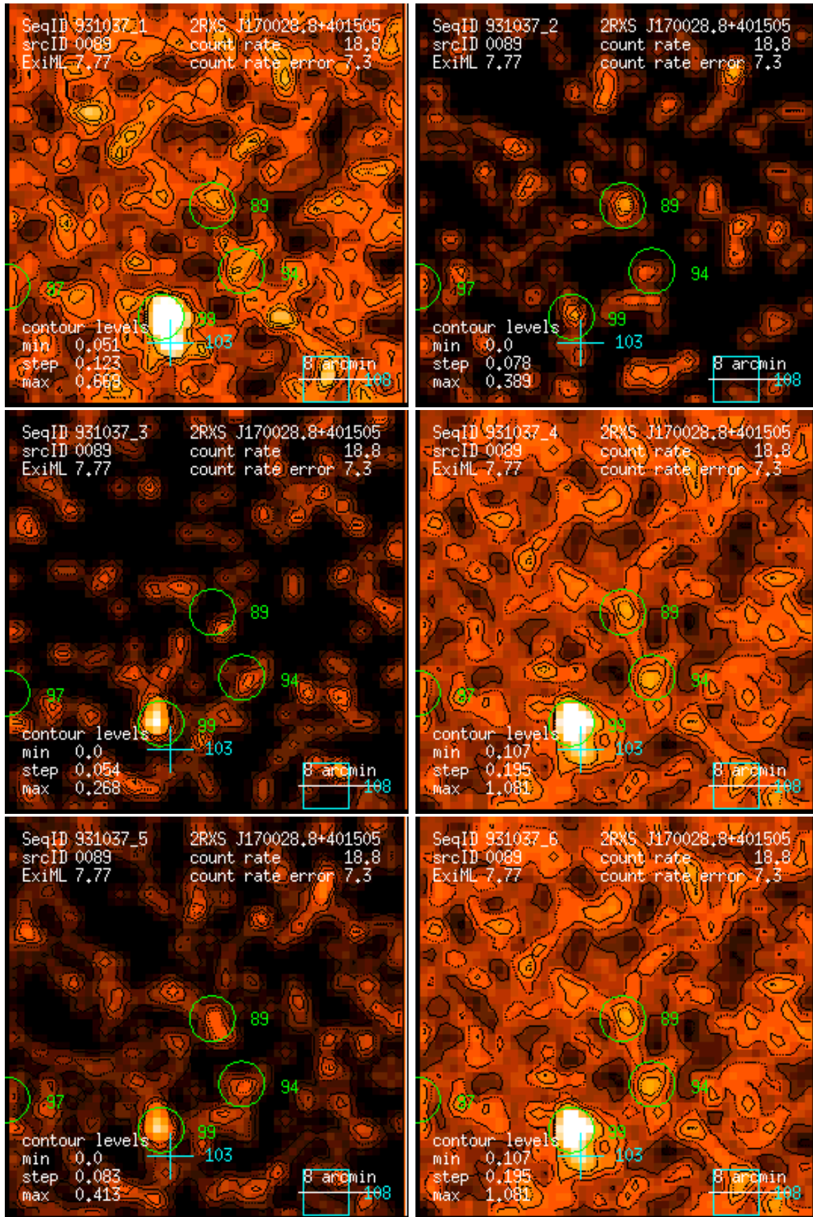
Figure 89: RASS 931037: detection 0089: band rate images, Gaussian filter: (1) PSPC channels 11 – 41, (2) 52 – 90, (3) 91 – 201, (4) 11 – 235, (5) 52 – 201, (6) 11 – 201. Broad band rates in counts/ks. Band rate contour levels in counts/ks/arcmin 2 .
