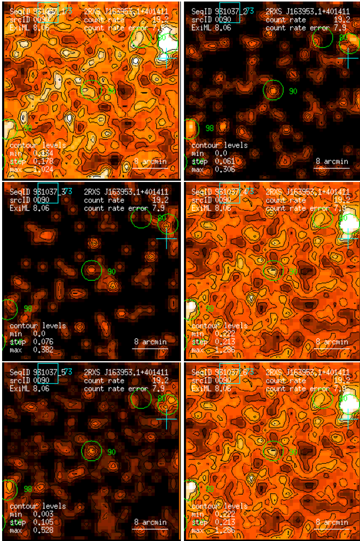
Figure 90: RASS 931037: detection 0090: band rate images, Gaussian filter: (1) PSPC channels 11 – 41, (2) 52 – 90, (3) 91 – 201, (4) 11 – 235, (5) 52 – 201, (6) 11 – 201. Broad band rates in counts/ks. Band rate contour levels in counts/ks/arcmin 2 .
