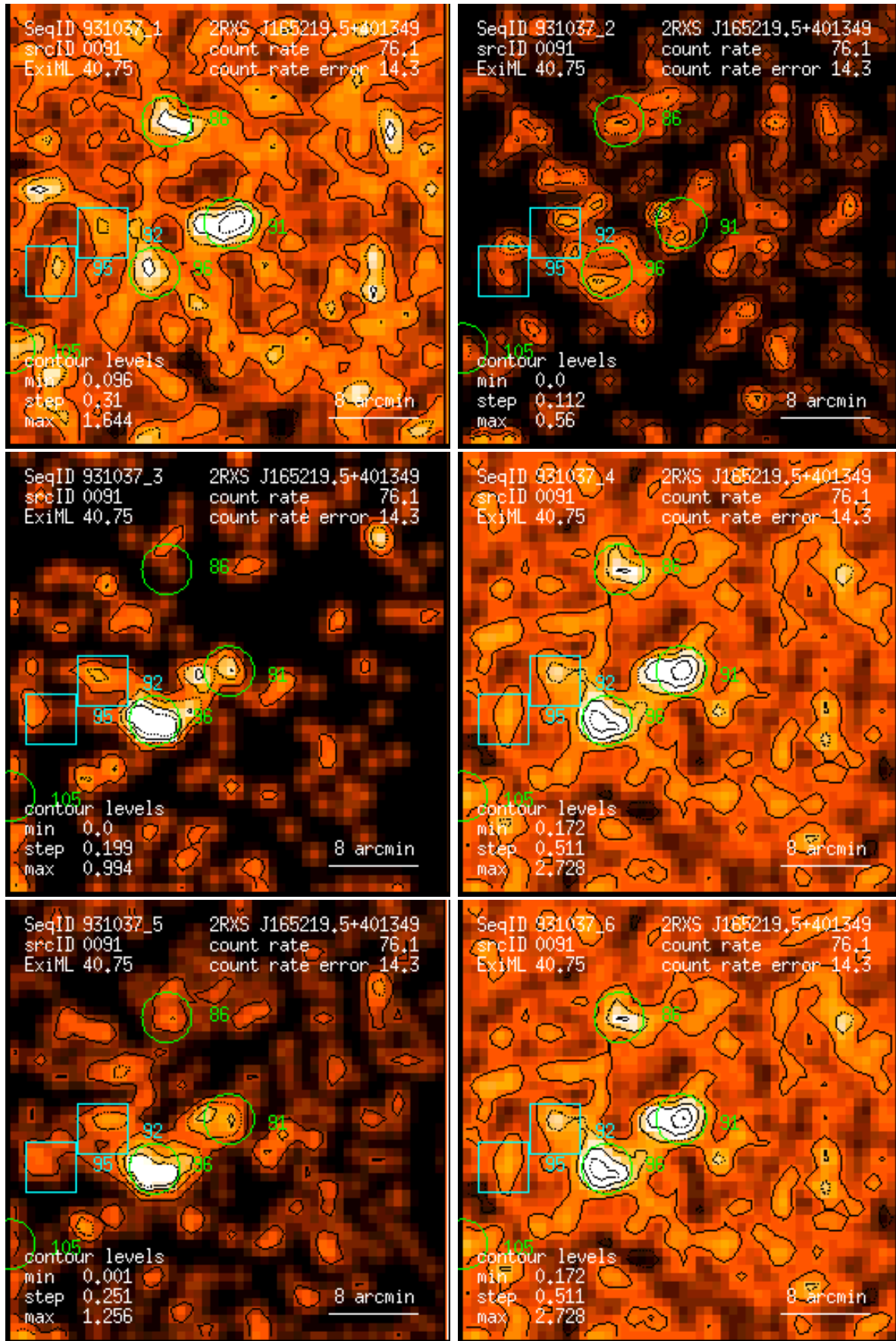
Figure 91: RASS 931037: detection 0091: band rate images, Gaussian filter: (1) PSPC channels 11 – 41, (2) 52 – 90, (3) 91 – 201, (4) 11 – 235, (5) 52 – 201, (6) 11 – 201. Broad band rates in counts/ks. Band rate contour levels in counts/ks/arcmin 2 .
