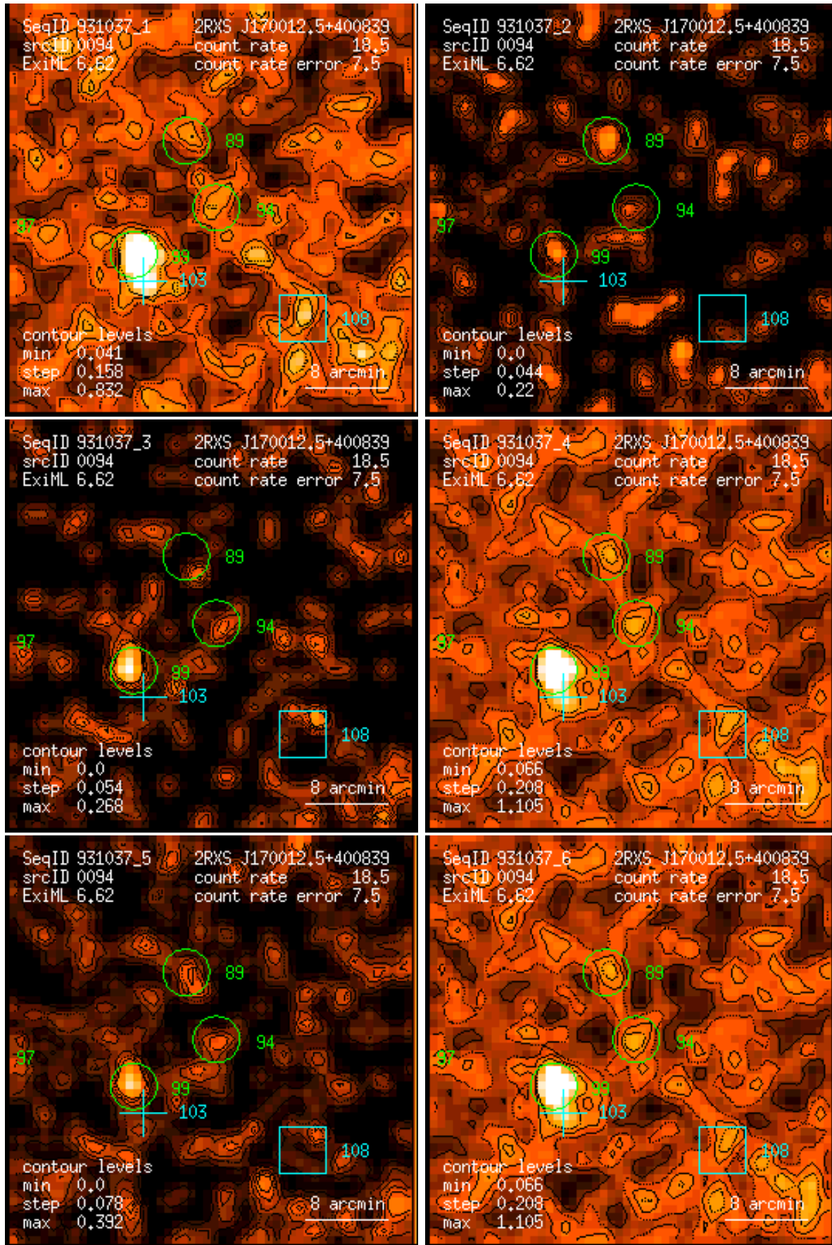
Figure 94: RASS 931037: detection 0094: band rate images, Gaussian filter: (1) PSPC channels 11 – 41, (2) 52 – 90, (3) 91 – 201, (4) 11 – 235, (5) 52 – 201, (6) 11 – 201. Broad band rates in counts/ks. Band rate contour levels in counts/ks/arcmin 2 .
