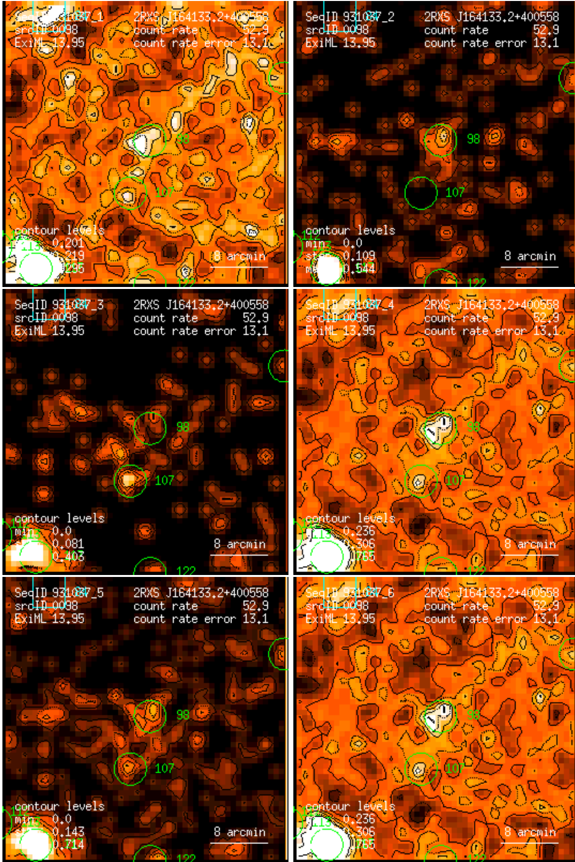
Figure 98: RASS 931037: detection 0098: band rate images, Gaussian filter: (1) PSPC channels 11 – 41, (2) 52 – 90, (3) 91 – 201, (4) 11 – 235, (5) 52 – 201, (6) 11 – 201. Broad band rates in counts/ks. Band rate contour levels in counts/ks/arcmin 2 .
