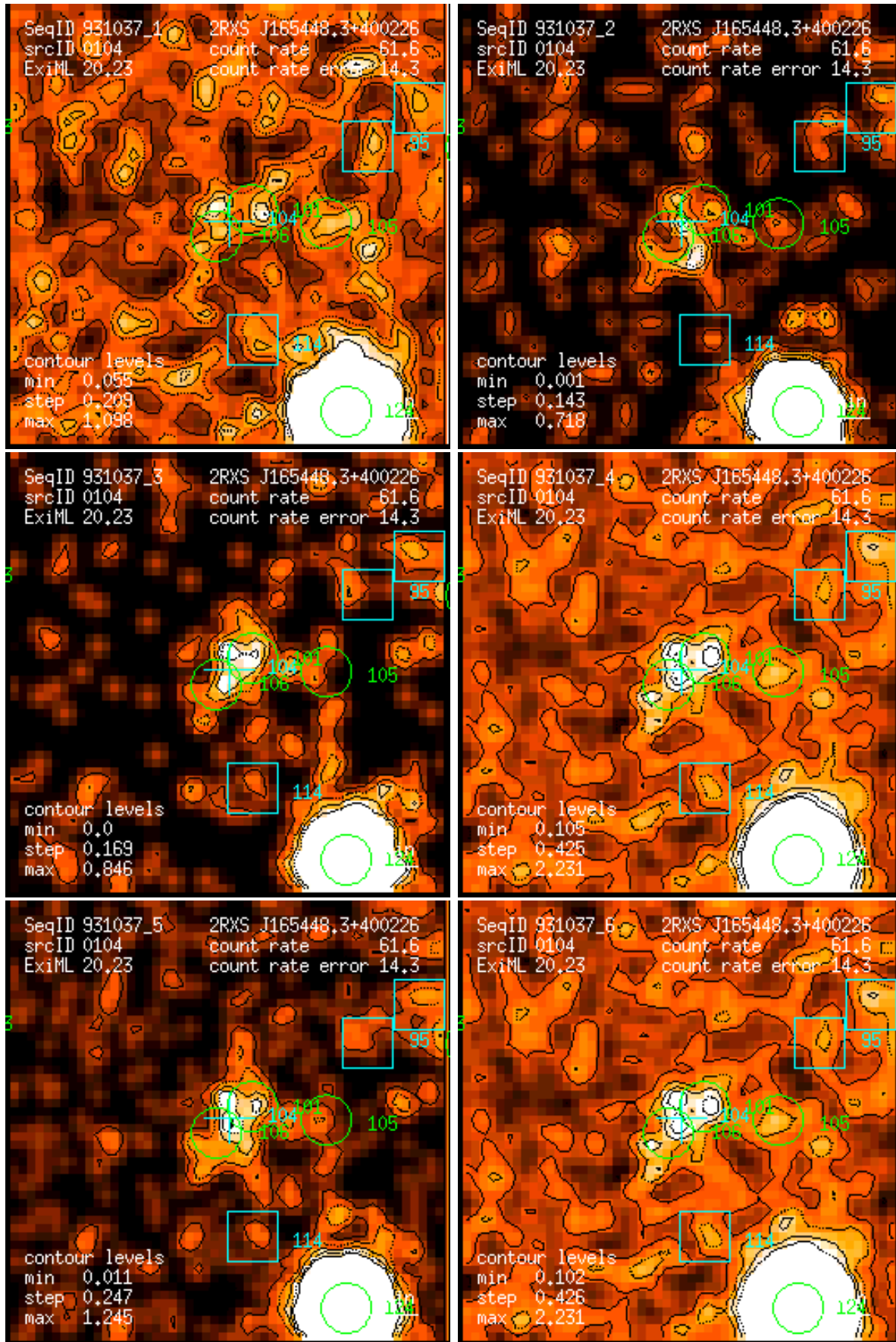
Figure 104: RASS 931037: detection 0104: band rate images, Gaussian filter: (1) PSPC channels 11 – 41, (2) 52 – 90, (3) 91 – 201, (4) 11 – 235, (5) 52 – 201, (6) 11 – 201. Broad band rates in counts/ks. Band rate contour levels in counts/ks/arcmin 2 .
