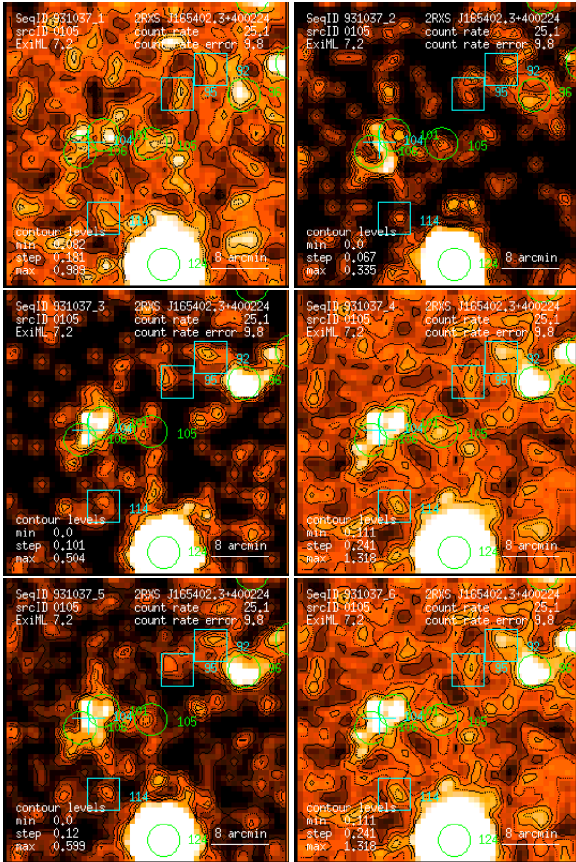
Figure 105: RASS 931037: detection 0105: band rate images, Gaussian filter: (1) PSPC channels 11 – 41, (2) 52 – 90, (3) 91 – 201, (4) 11 – 235, (5) 52 – 201, (6) 11 – 201. Broad band rates in counts/ks. Band rate contour levels in counts/ks/arcmin 2 .
