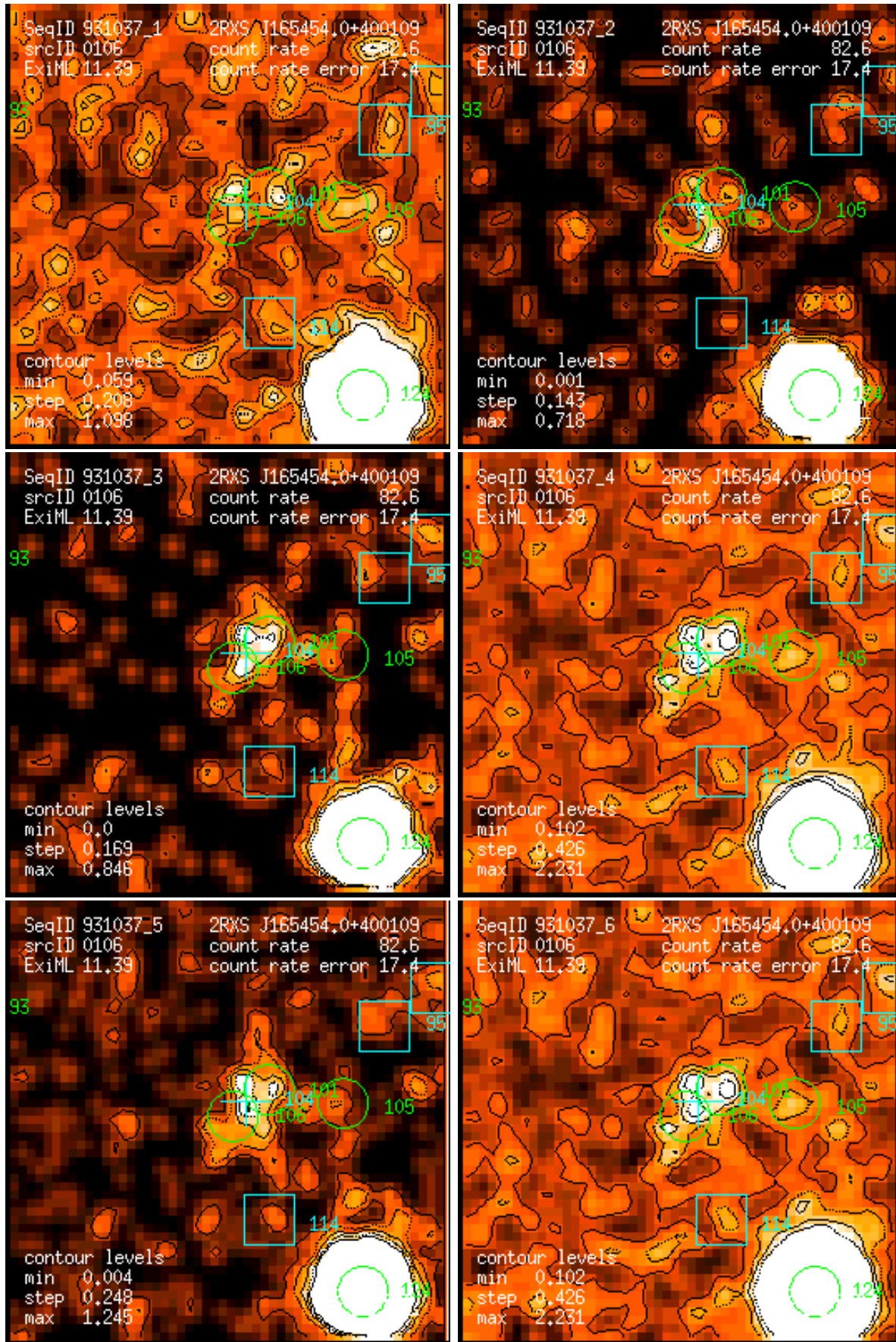
Figure 106: RASS 931037: detection 0106: band rate images, Gaussian filter: (1) PSPC channels 11 – 41, (2) 52 – 90, (3) 91 – 201, (4) 11 – 235, (5) 52 – 201, (6) 11 – 201. Broad band rates in counts/ks. Band rate contour levels in counts/ks/arcmin 2 .
