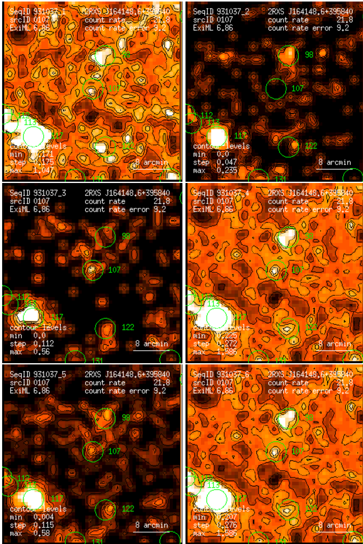
Figure 107: RASS 931037: detection 0107: band rate images, Gaussian filter: (1) PSPC channels 11 – 41, (2) 52 – 90, (3) 91 – 201, (4) 11 – 235, (5) 52 – 201, (6) 11 – 201. Broad band rates in counts/ks. Band rate contour levels in counts/ks/arcmin 2 .
