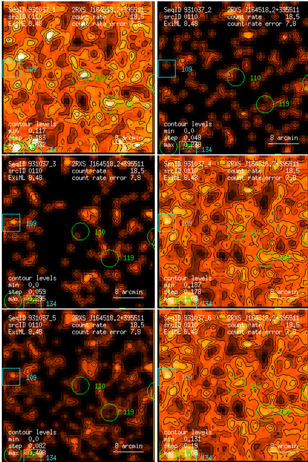
Figure 110: RASS 931037: detection 0110: band rate images, Gaussian filter: (1) PSPC channels 11 – 41, (2) 52 – 90, (3) 91 – 201, (4) 11 – 235, (5) 52 – 201, (6) 11 – 201. Broad band rates in counts/ks. Band rate contour levels in counts/ks/arcmin 2 .
